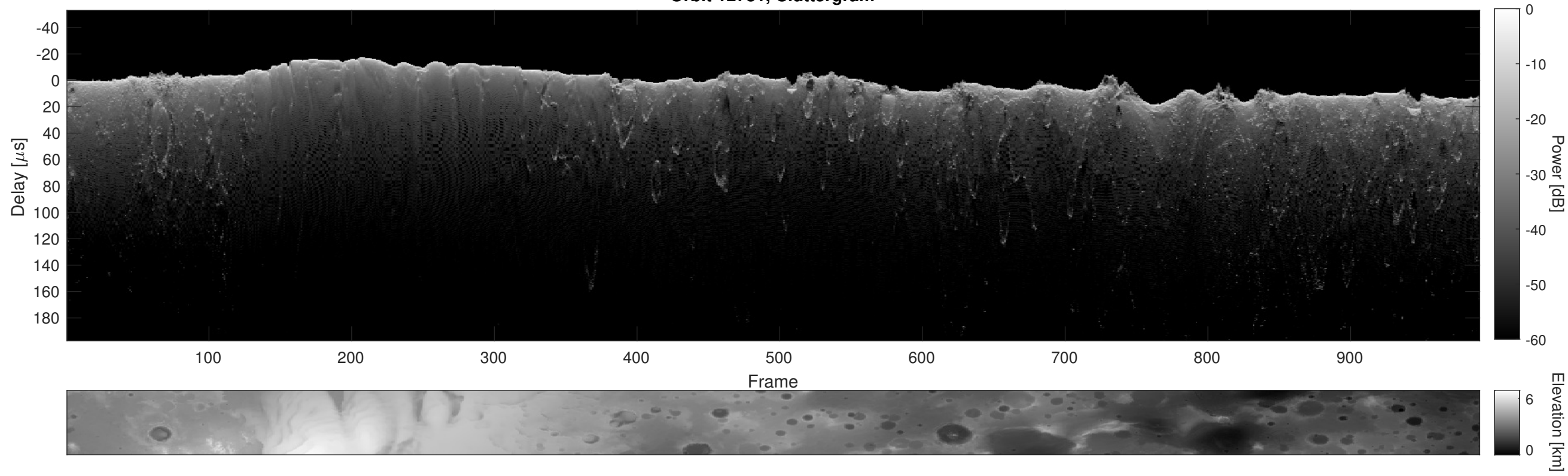
Orbit 12731, Cluttergram
