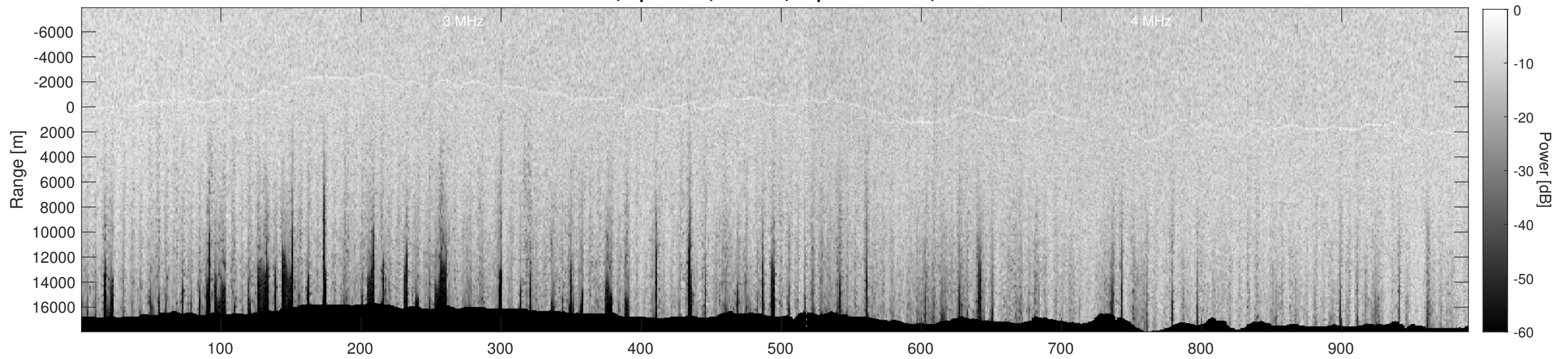
Orbit 12731, Depth-Corrected Cluttergram
