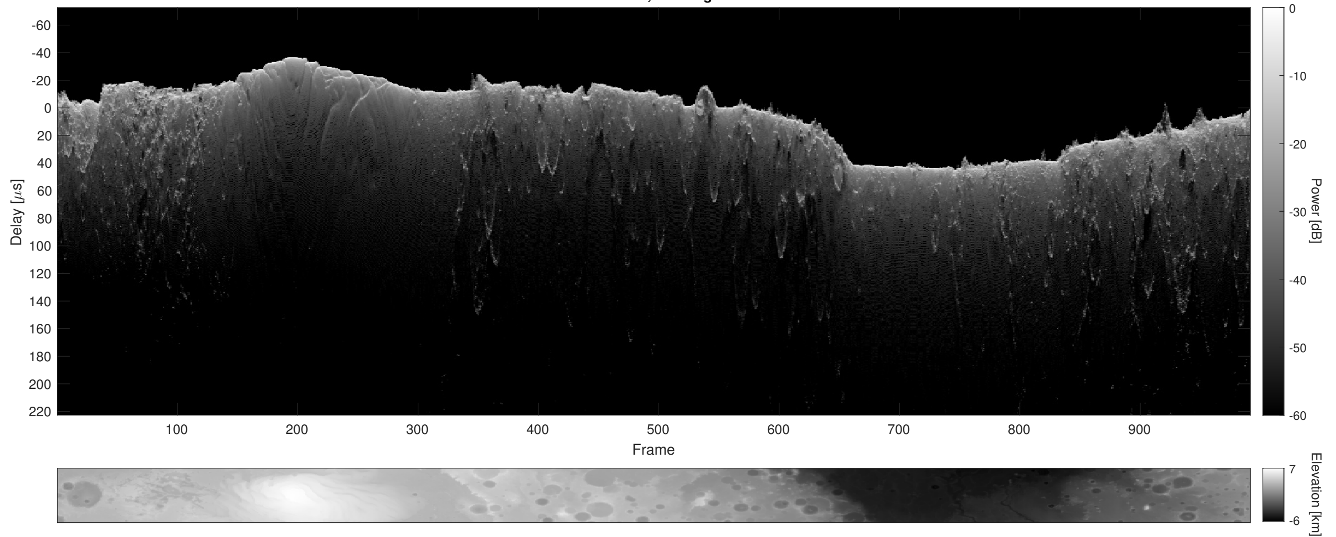
Orbit 12732, Cluttergram
