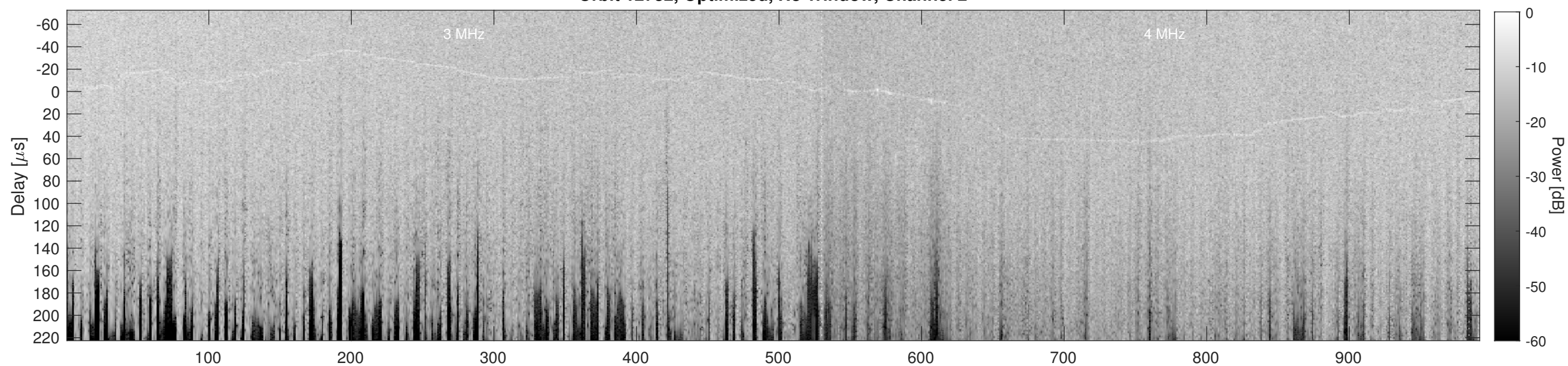
Orbit 12732, Cluttergram
