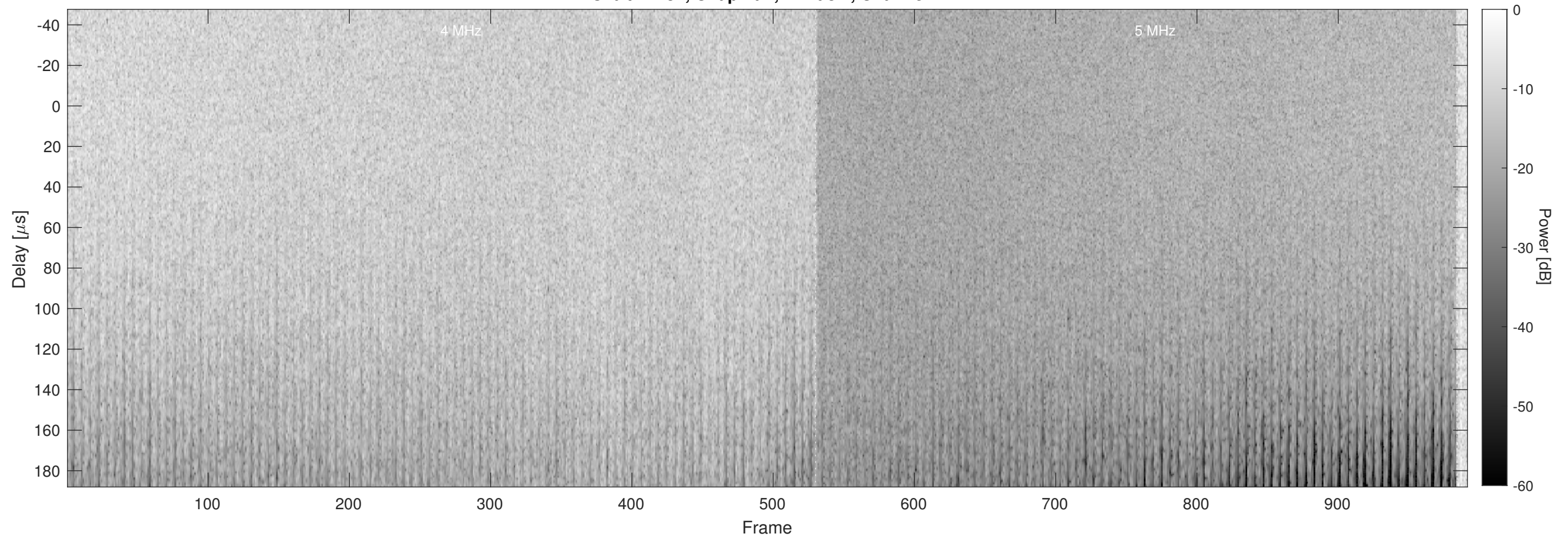
Orbit 12734, Chapman, Window, Channel 2
