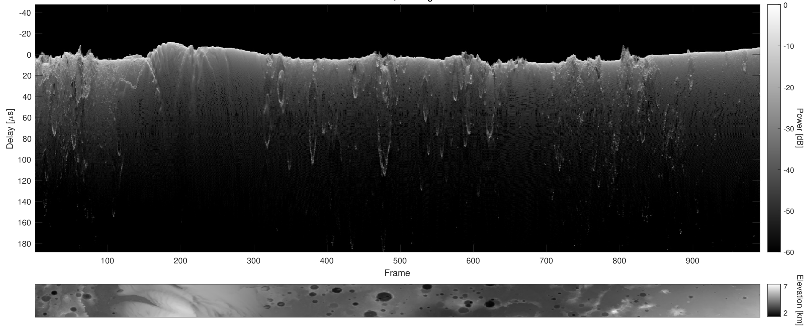
Orbit 12734, Cluttergram
