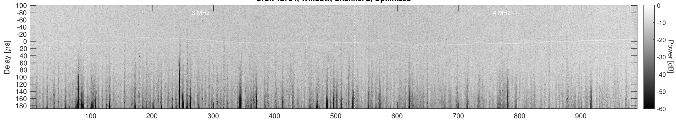
Orbit 12734, Cluttergram
