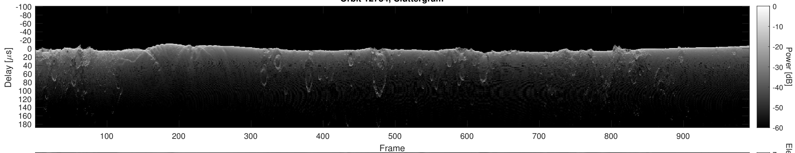
Orbit 12734, Cluttergram
