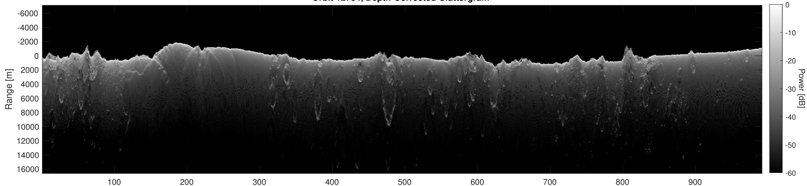
Orbit 12734, Depth-Corrected Cluttergram
