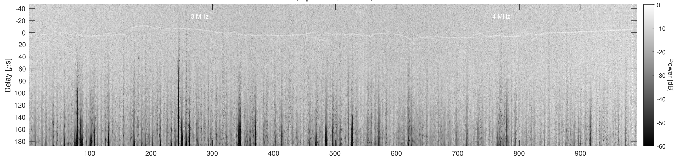
Orbit 12734, Cluttergram
