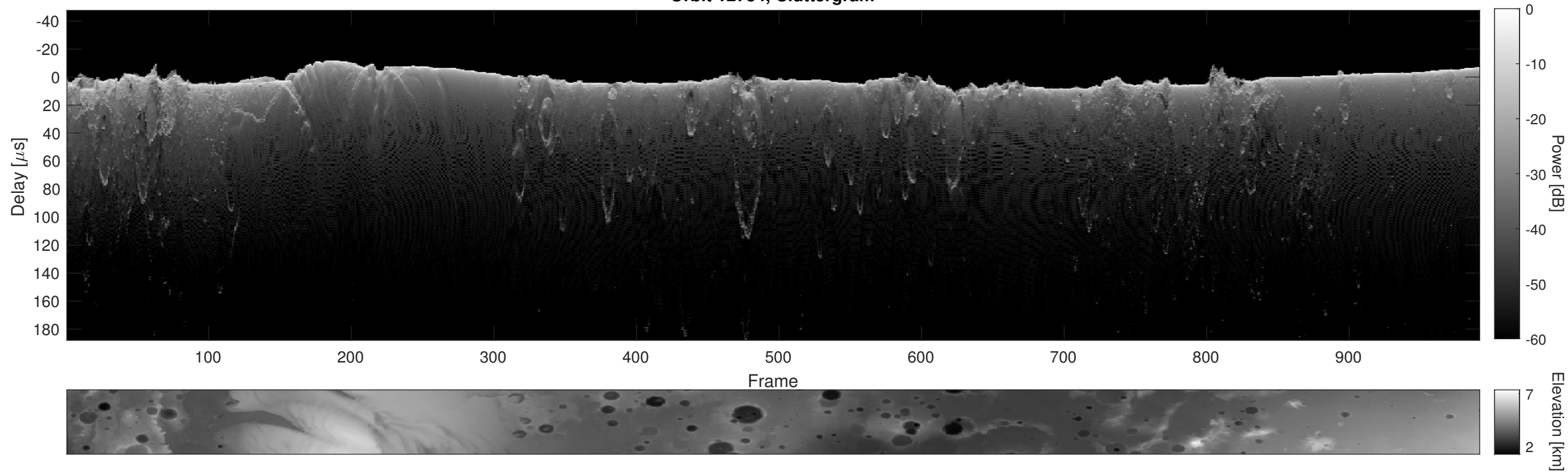
Orbit 12734, Cluttergram
