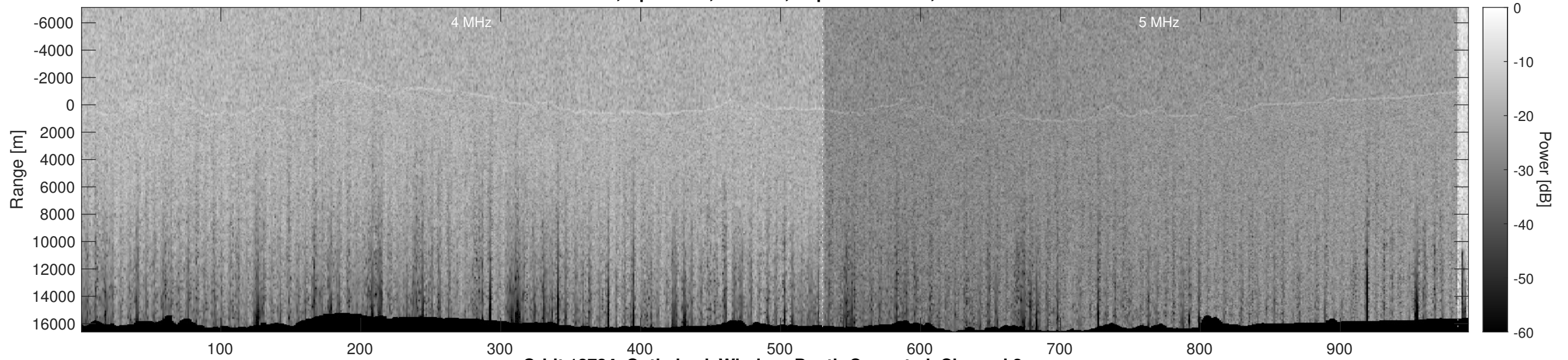
Orbit 12734, Optimized, Window, Depth-Corrected, Channel 2
