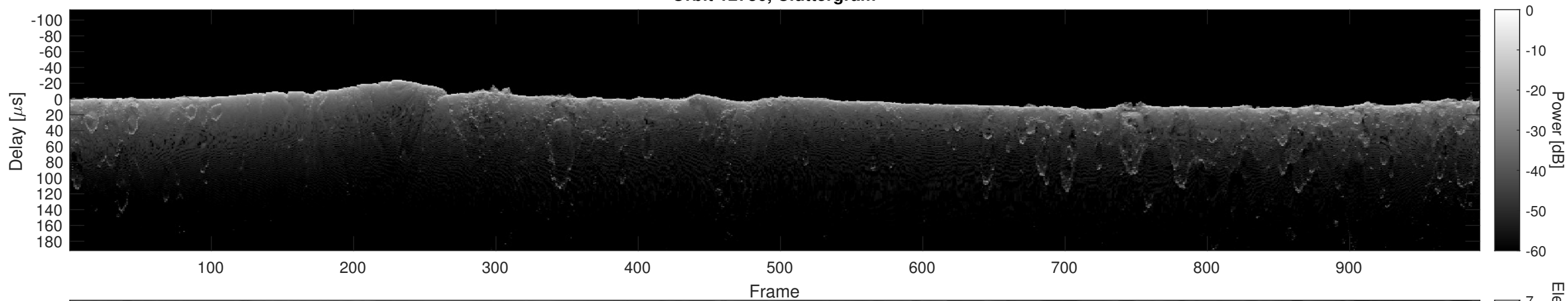
Orbit 12736, Cluttergram
