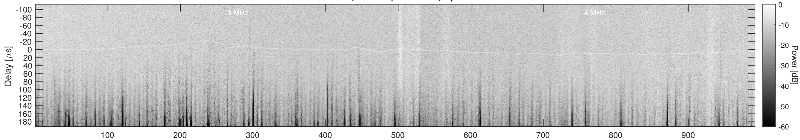
Orbit 12736, Cluttergram
