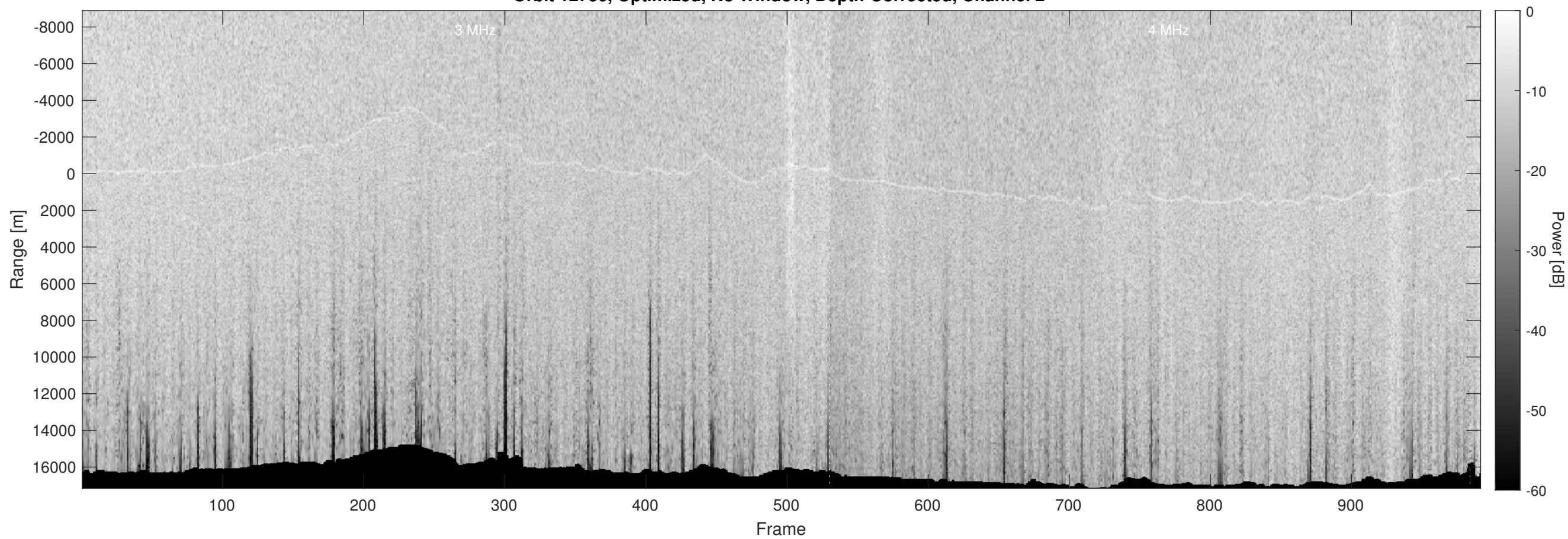
Orbit 12736, Optimized, No Window, Depth-Corrected, Channel 2
