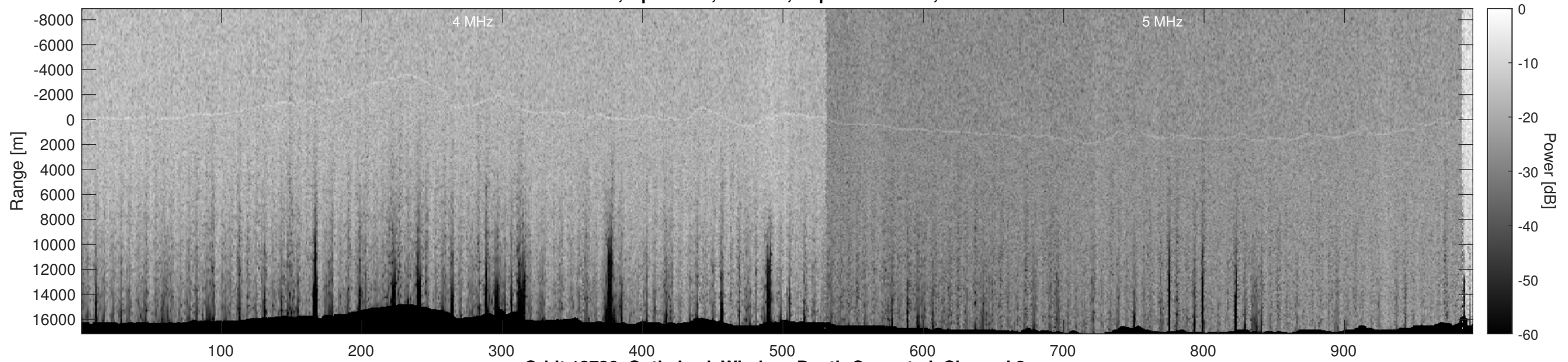
Orbit 12736, Optimized, Window, Depth-Corrected, Channel 2
