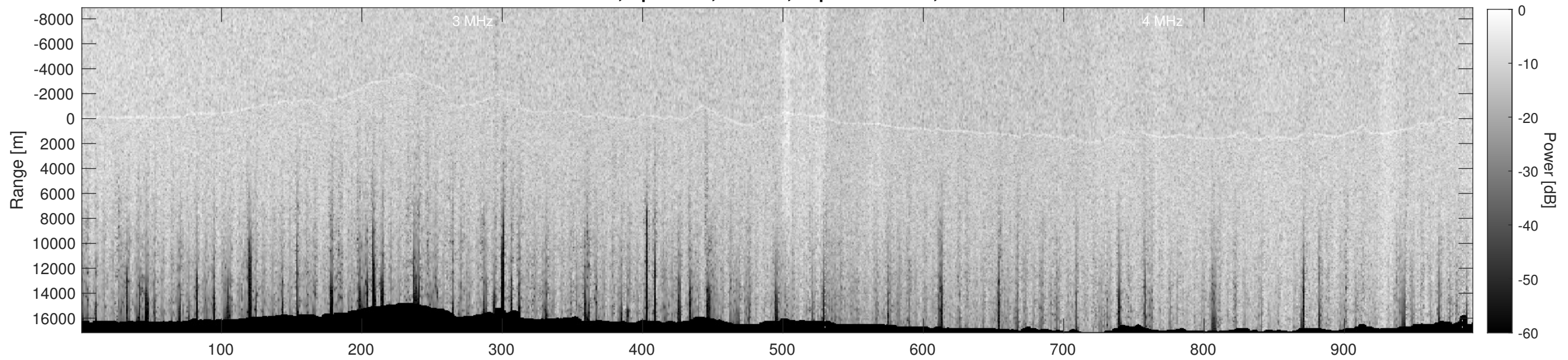
Orbit 12736, Depth-Corrected Cluttergram
