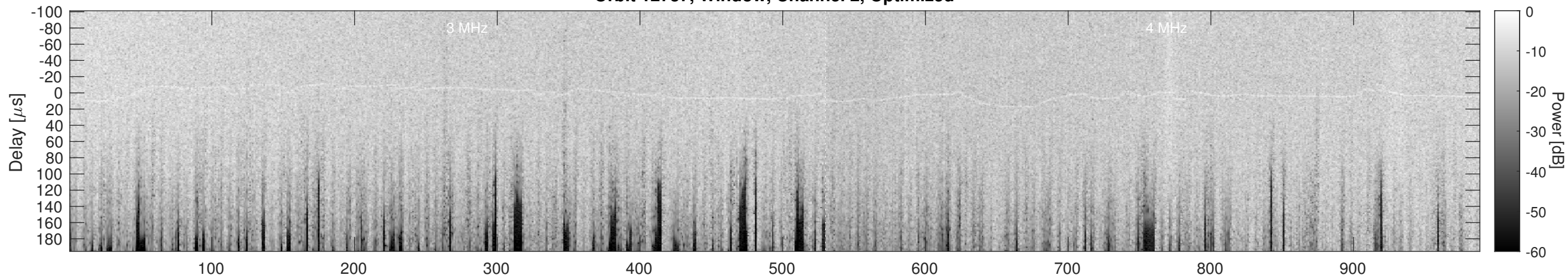
Orbit 12737, Cluttergram
