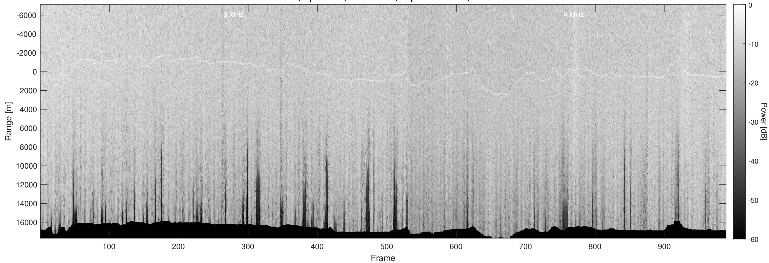
Orbit 12737, Optimized, No Window, Depth-Corrected, Channel 2
