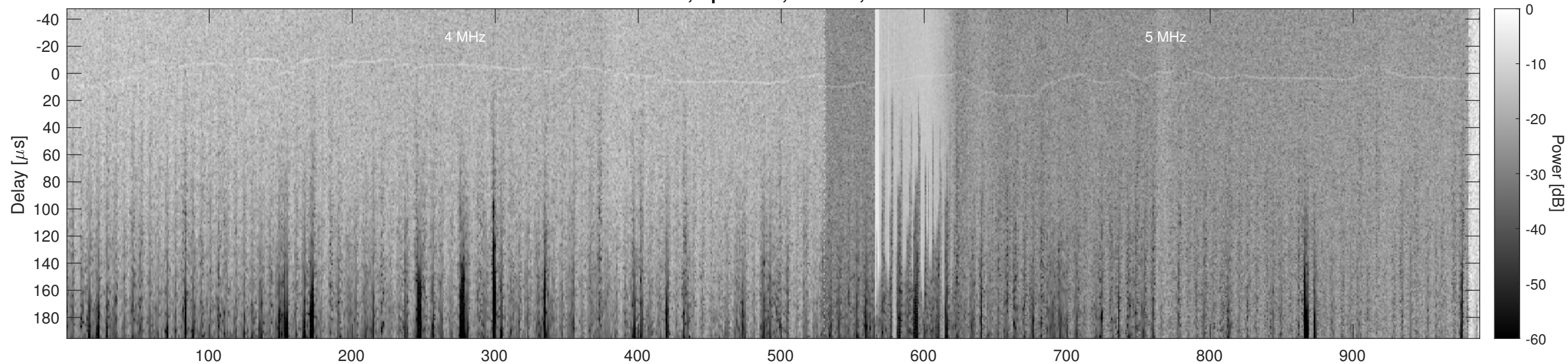
Orbit 12737, Optimized, Window, Channel 2
