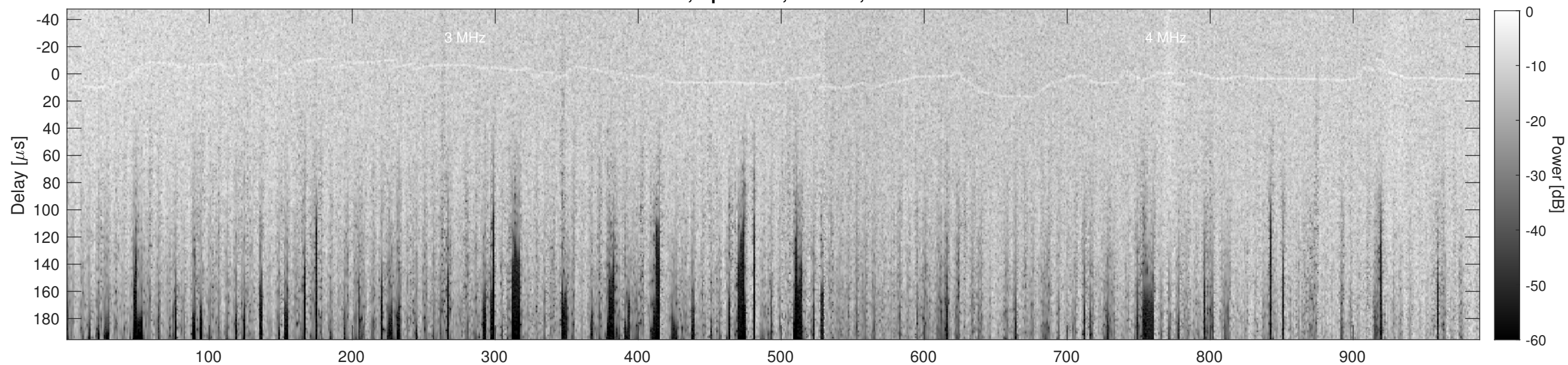
Orbit 12737, Cluttergram
