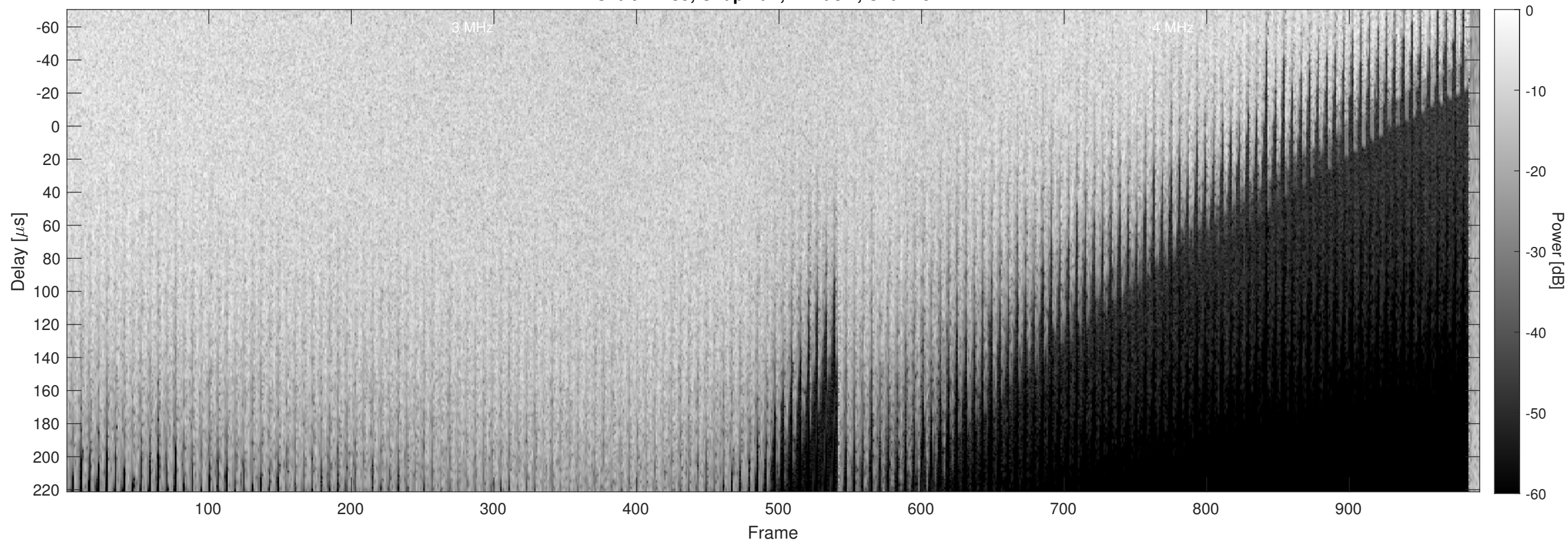
Orbit 12739, Chapman, Window, Channel 2
