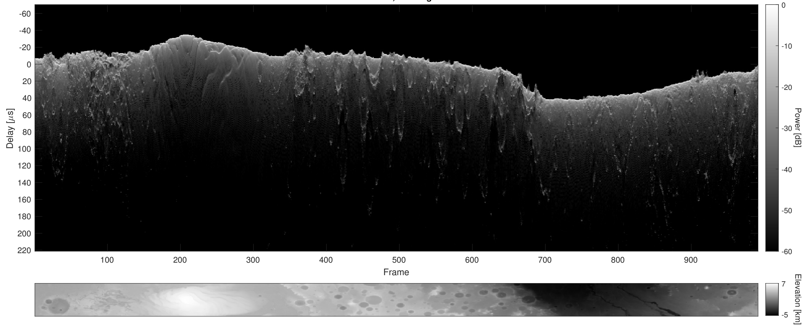
Orbit 12739, Cluttergram
