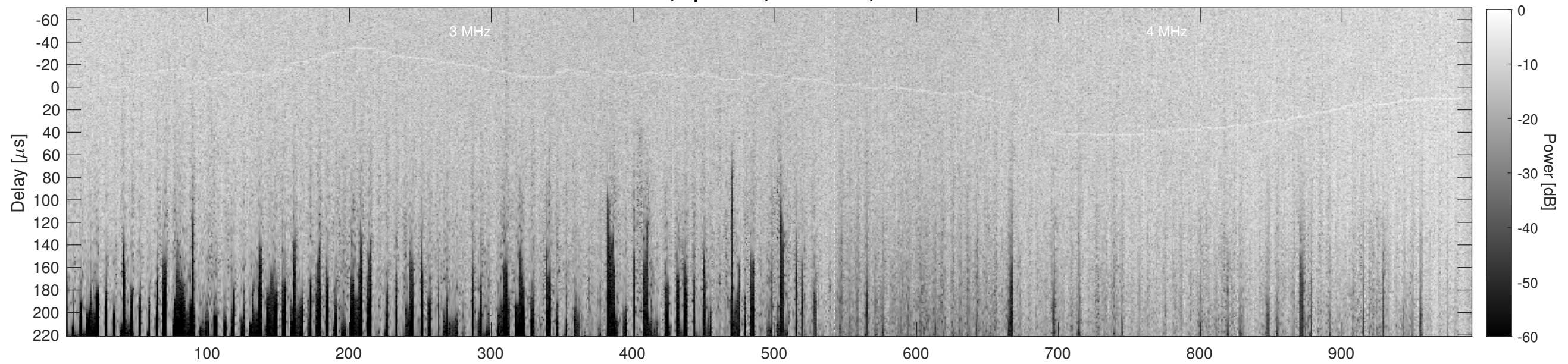
Orbit 12739, Cluttergram
