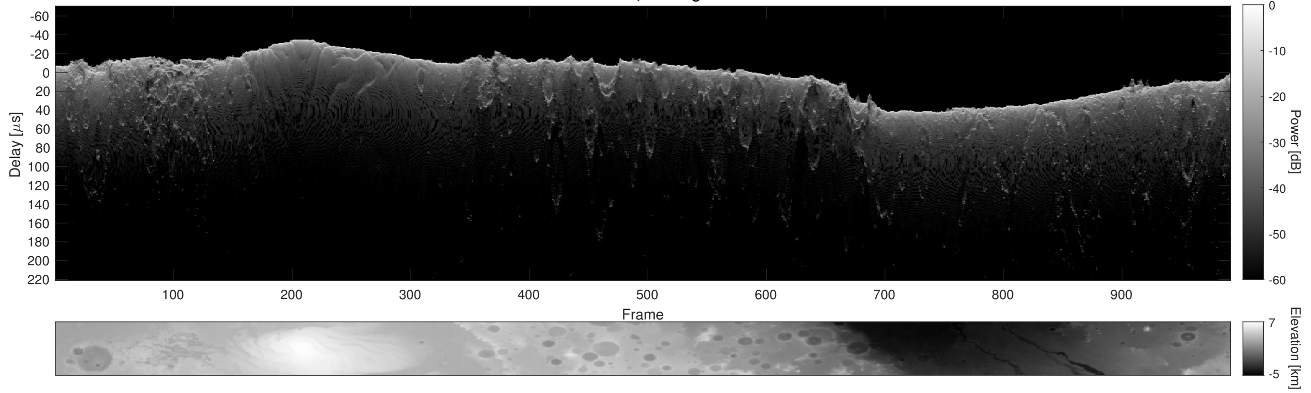
Orbit 12739, Cluttergram
