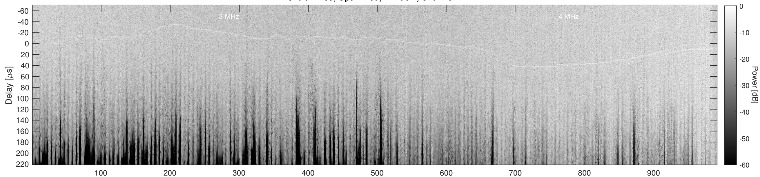
Orbit 12739, Cluttergram
