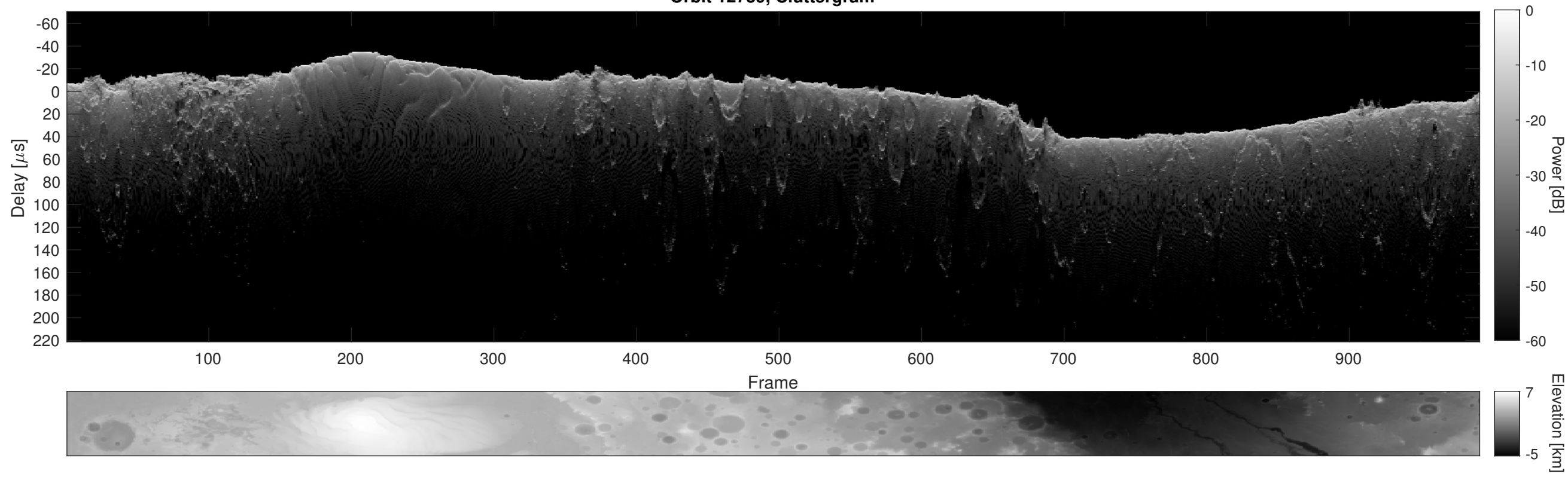
Orbit 12739, Cluttergram
