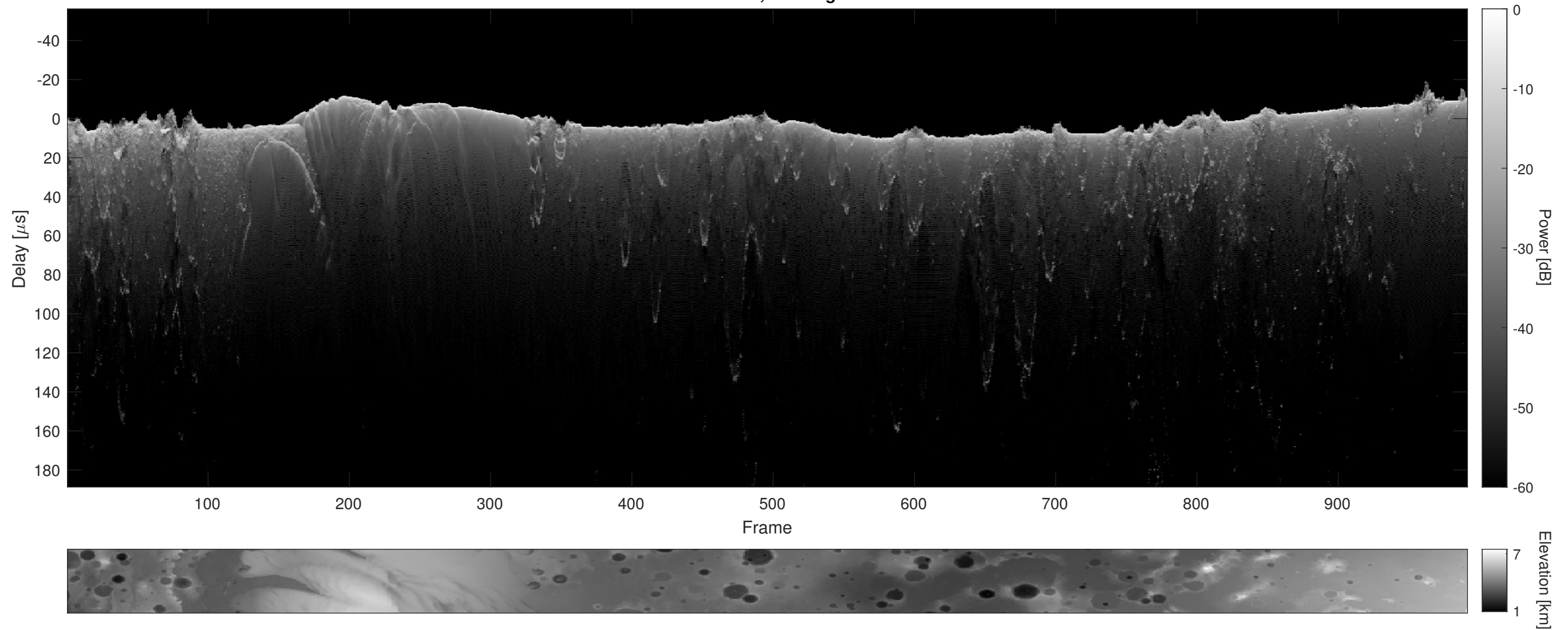
Orbit 12741, Cluttergram
