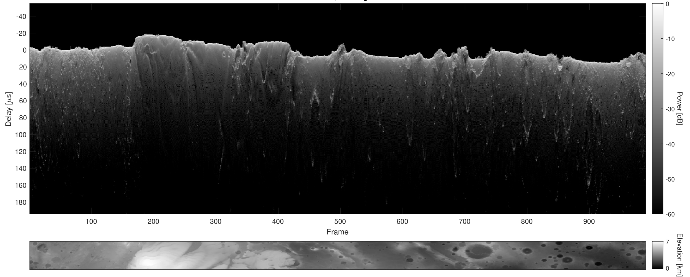
Orbit 12742, Cluttergram
