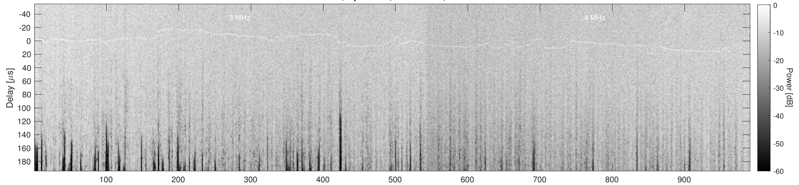
Orbit 12742, Cluttergram
