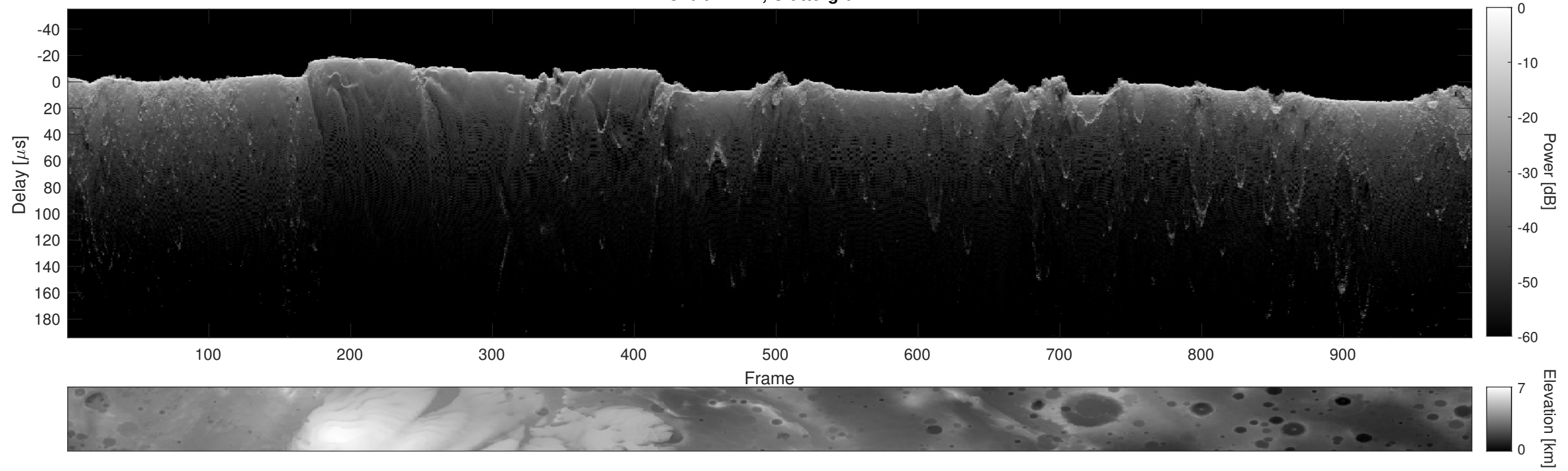
Orbit 12742, Cluttergram
