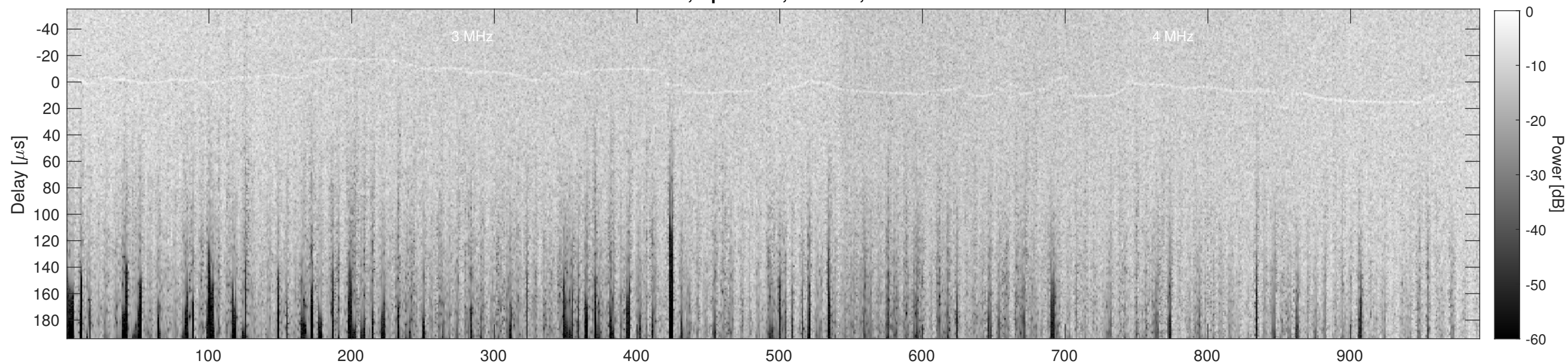
Orbit 12742, Cluttergram
