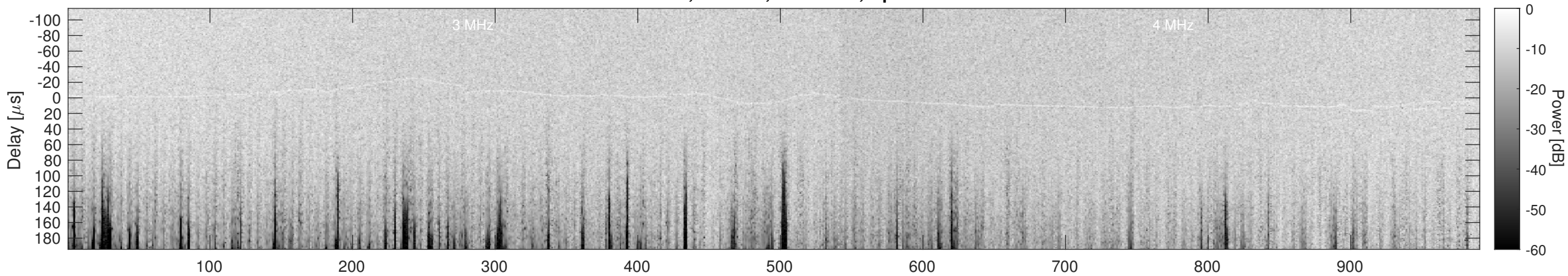
Orbit 12743, Cluttergram
