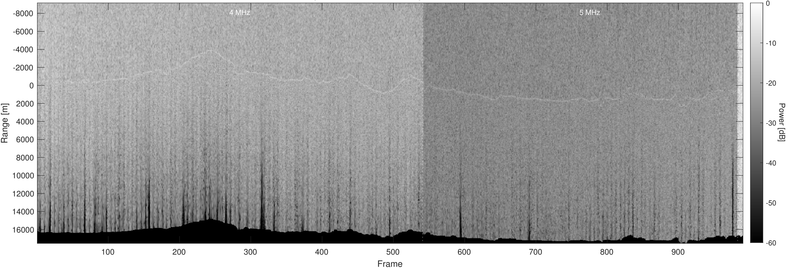
Orbit 12743, Optimized, No Window, Depth-Corrected, Channel 2
