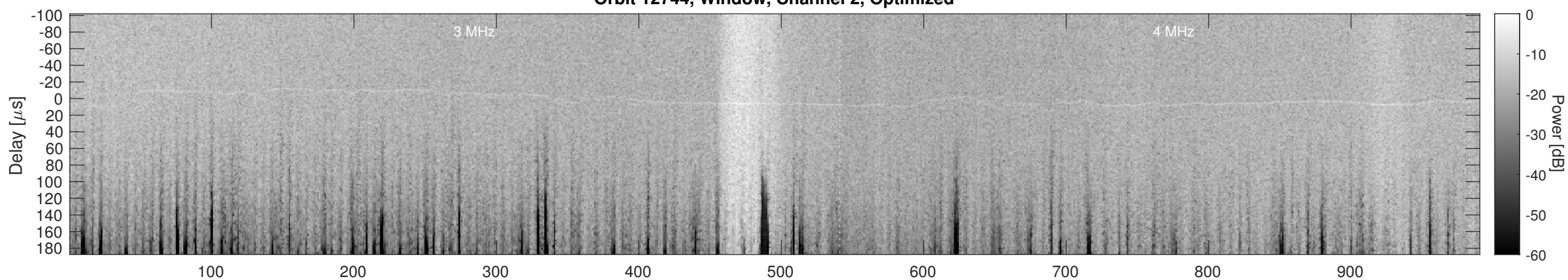
Orbit 12744, Cluttergram
