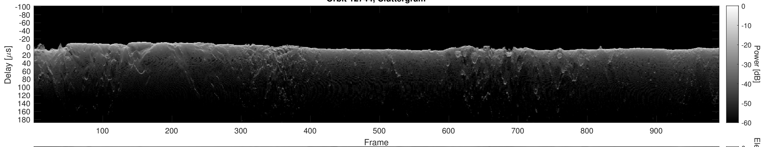
Orbit 12744, Cluttergram
