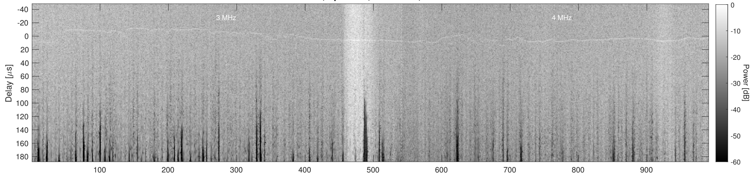
Orbit 12744, Cluttergram
