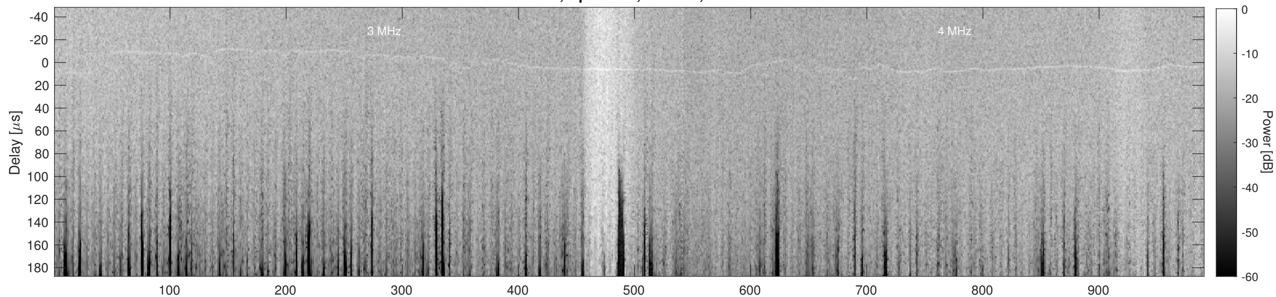
Orbit 12744, Cluttergram
