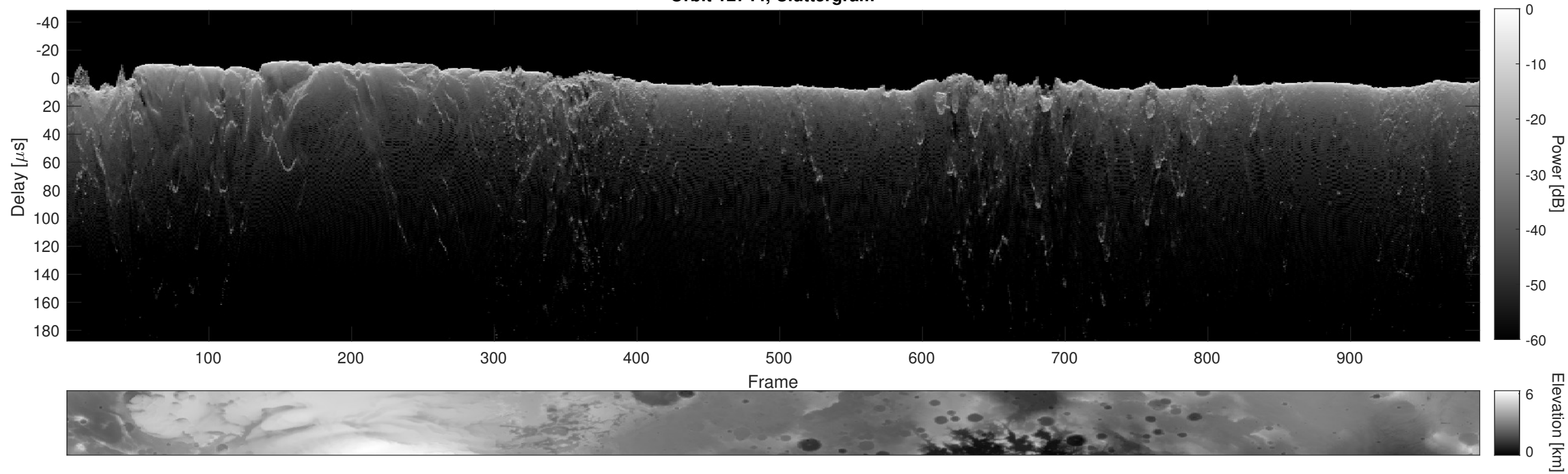
Orbit 12744, Cluttergram
