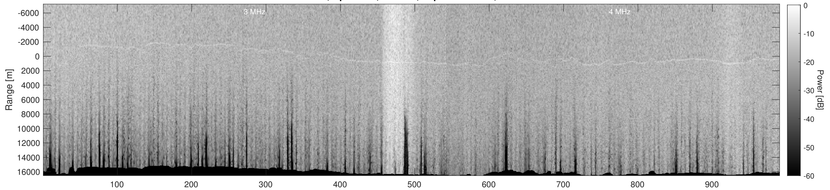
Orbit 12744, Depth-Corrected Cluttergram
