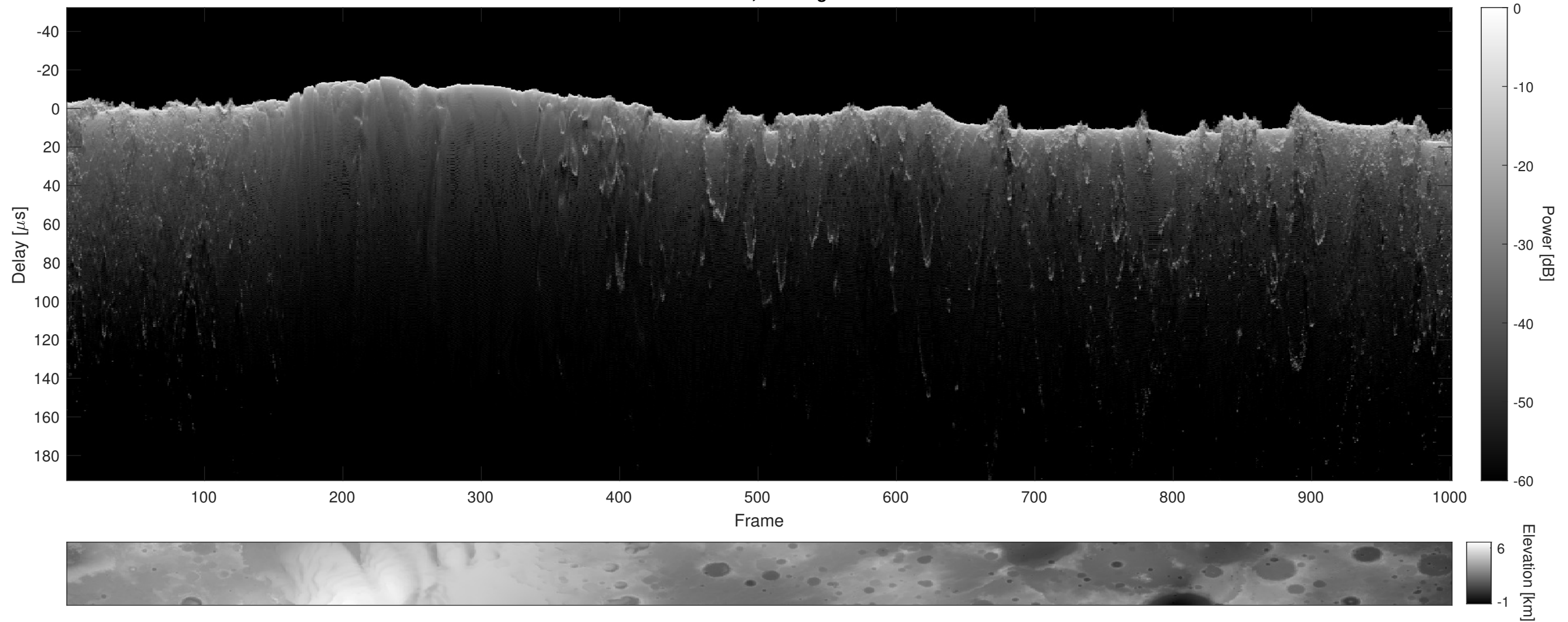
Orbit 12745, Cluttergram
