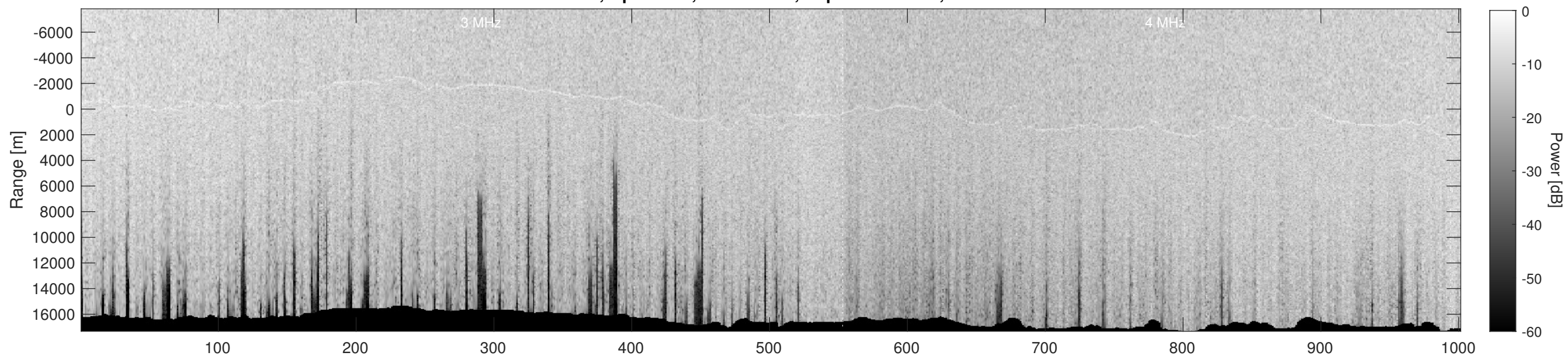
Orbit 12745, Depth-Corrected Cluttergram
