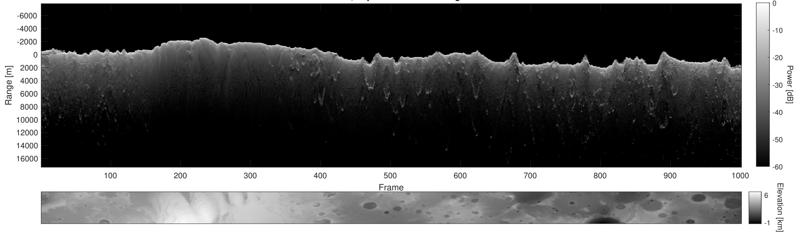
Orbit 12745, Depth-Corrected Cluttergram
