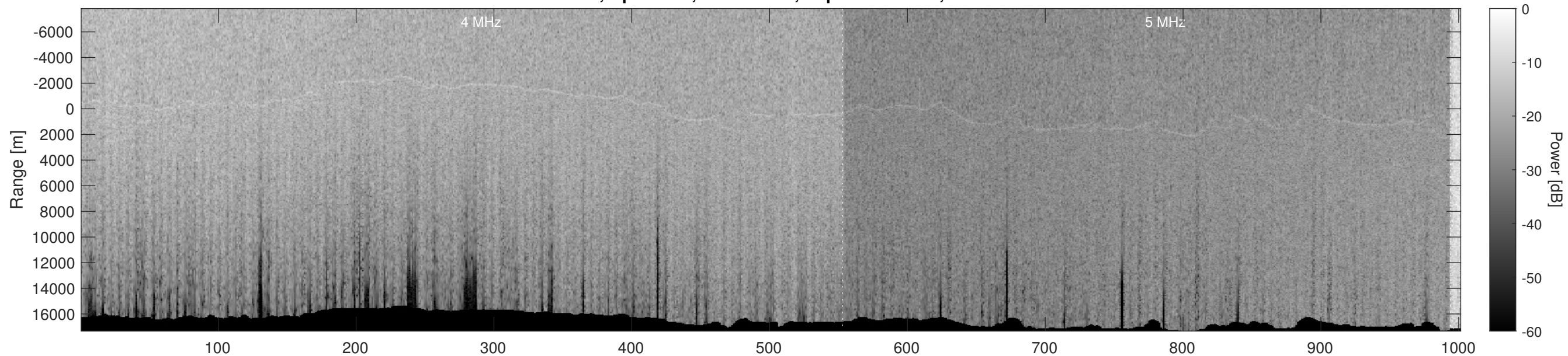
Orbit 12745, Optimized, No Window, Depth-Corrected, Channel 2
