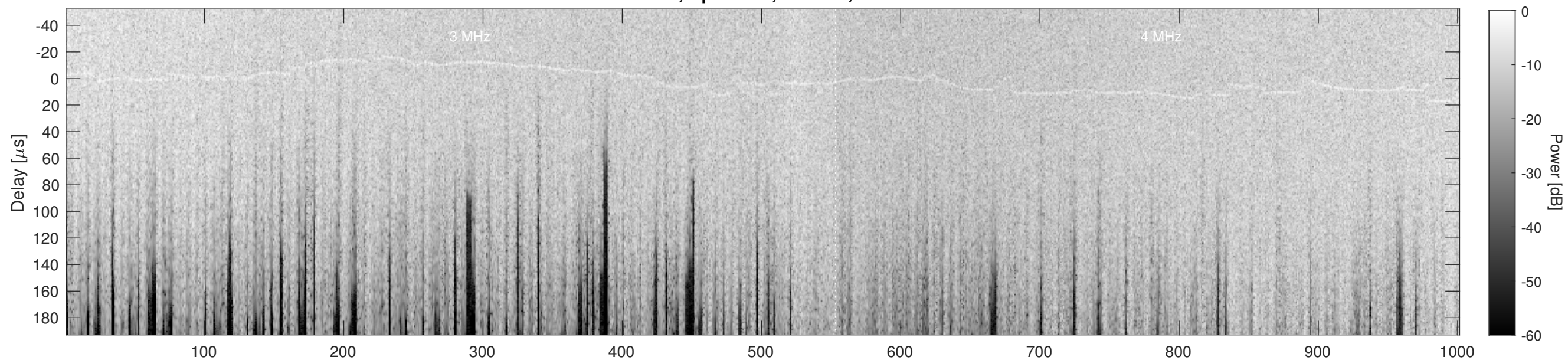
Orbit 12745, Cluttergram
