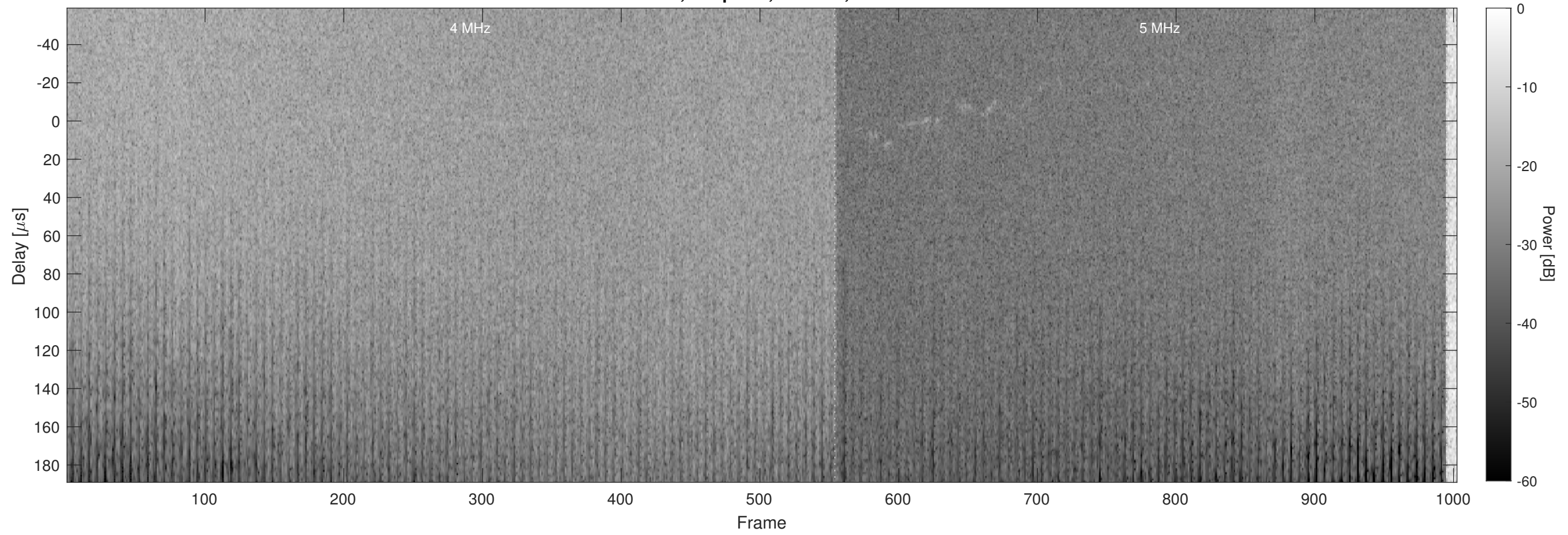
Orbit 12748, Chapman, Window, Channel 2
