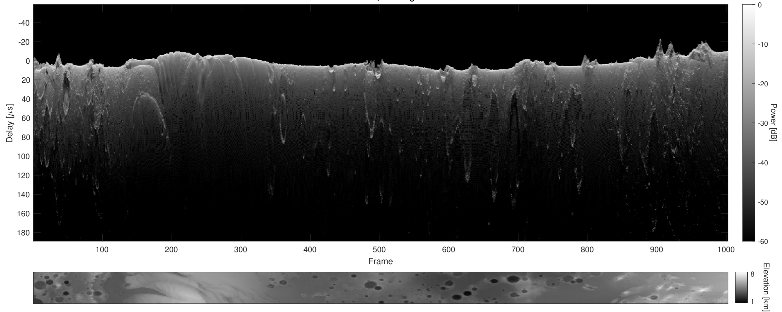
Orbit 12748, Cluttergram
