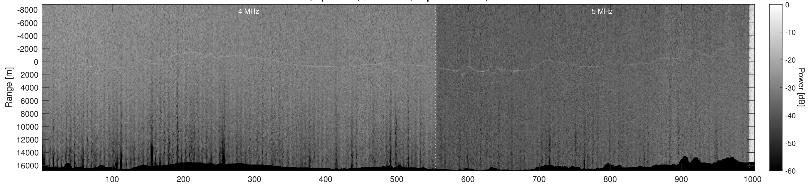
Orbit 12748, Optimized, No Window, Depth-Corrected, Channel 2
