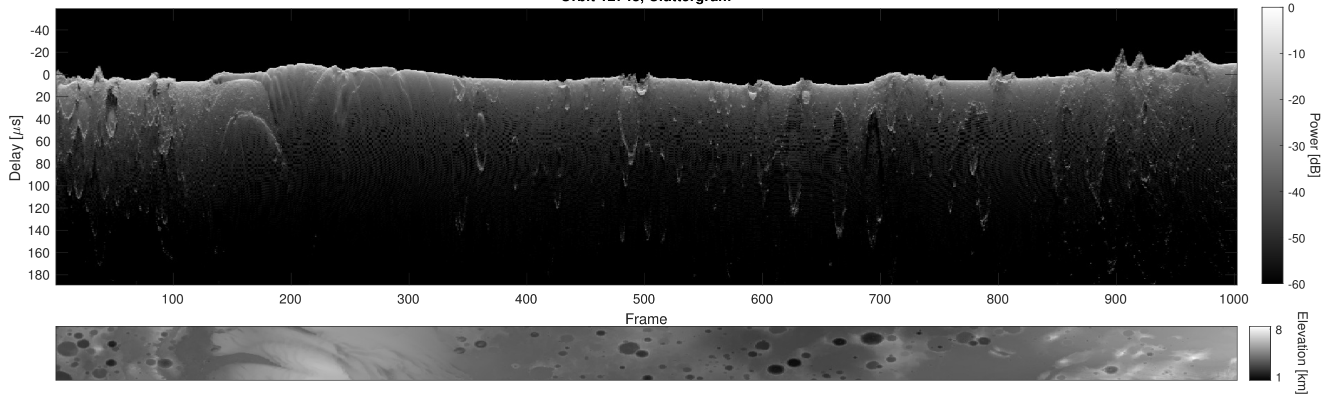
Orbit 12748, Cluttergram
