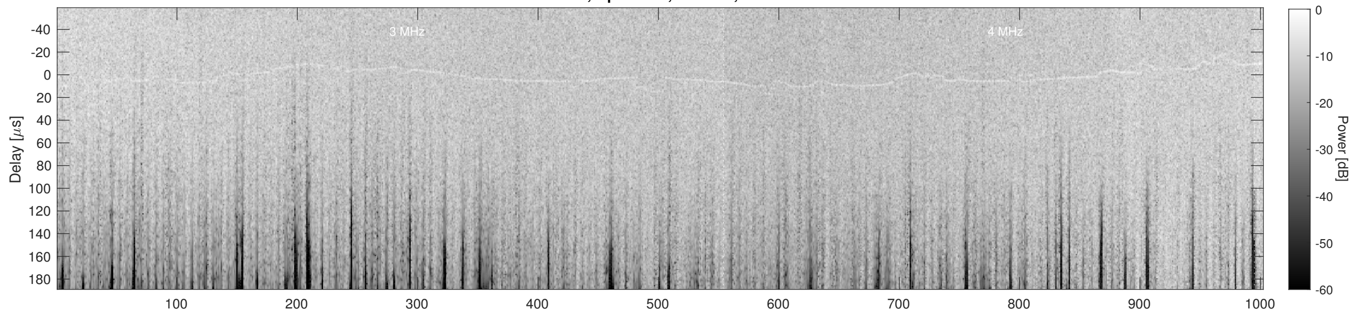
Orbit 12748, Cluttergram
