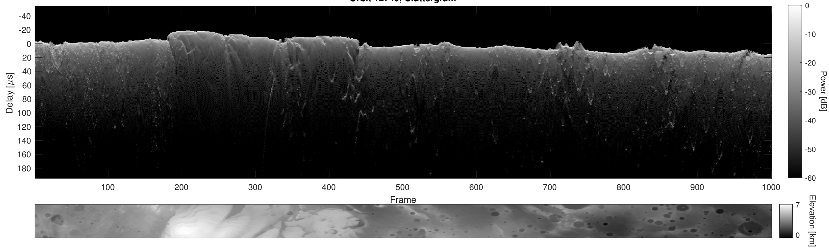
Orbit 12749, Cluttergram
