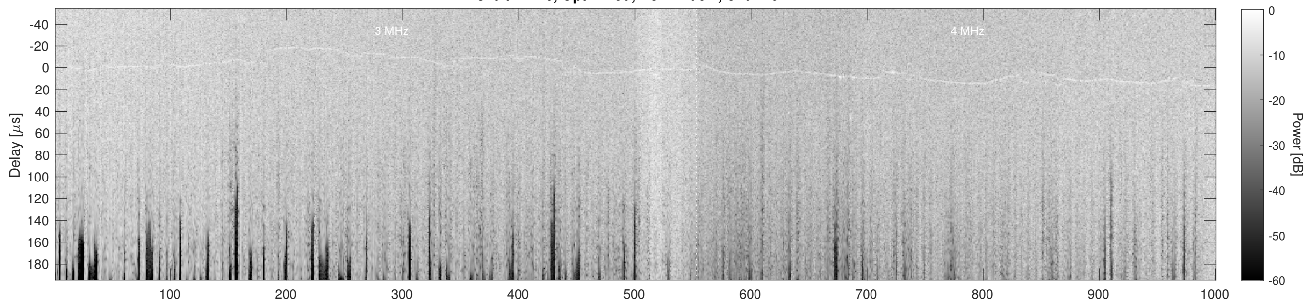
Orbit 12749, Cluttergram
