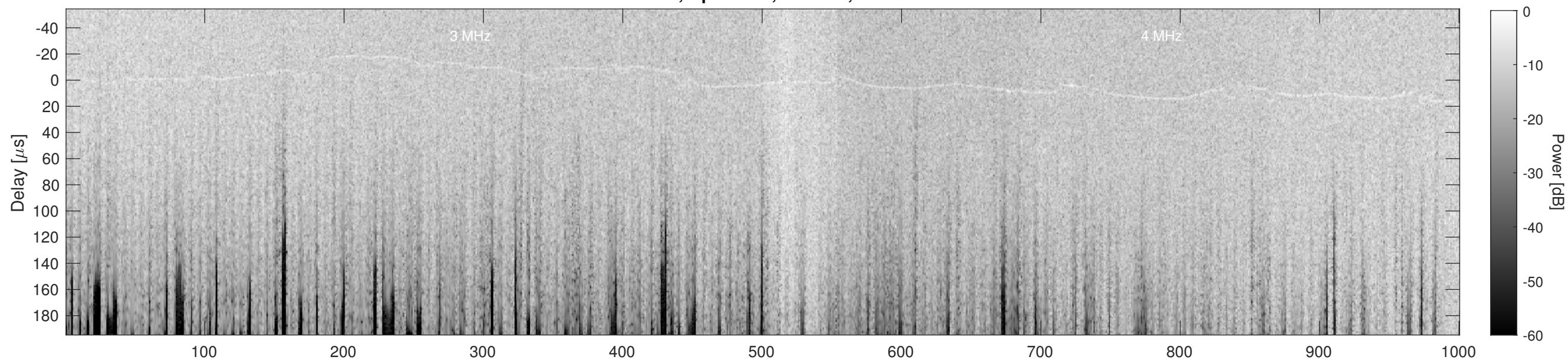
Orbit 12749, Cluttergram
