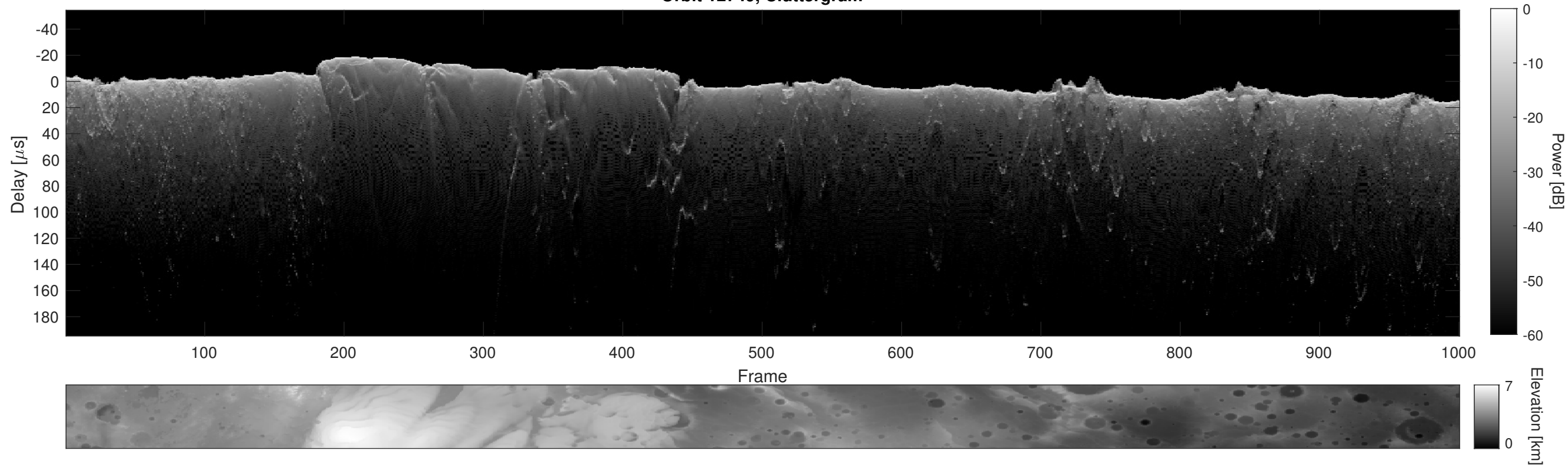
Orbit 12749, Cluttergram
