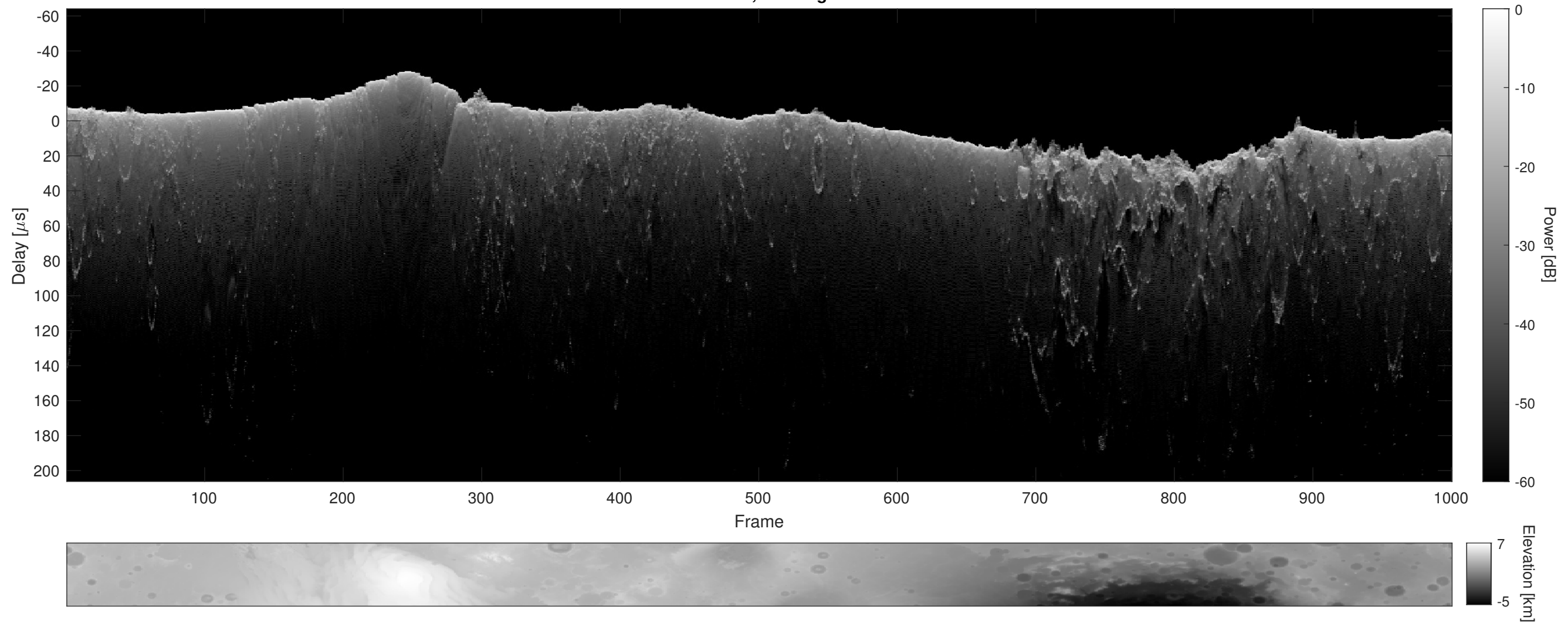
Orbit 12750, Cluttergram
