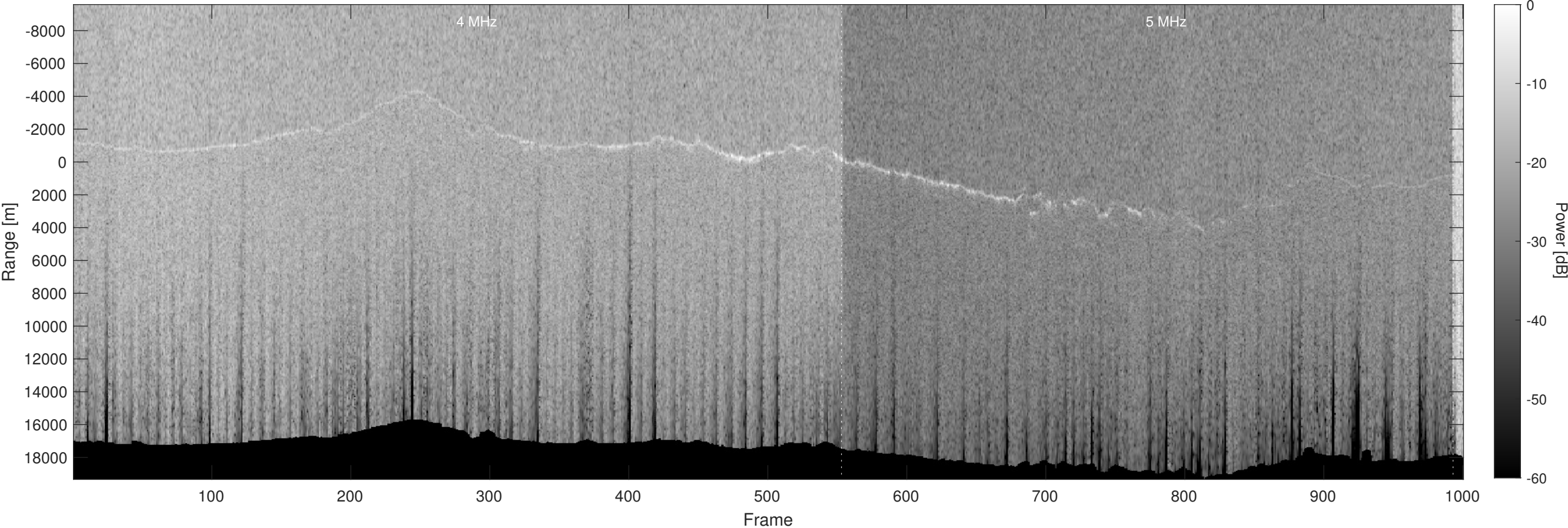
Orbit 12750, Optimized, Window, Depth-Corrected, Channel 2
