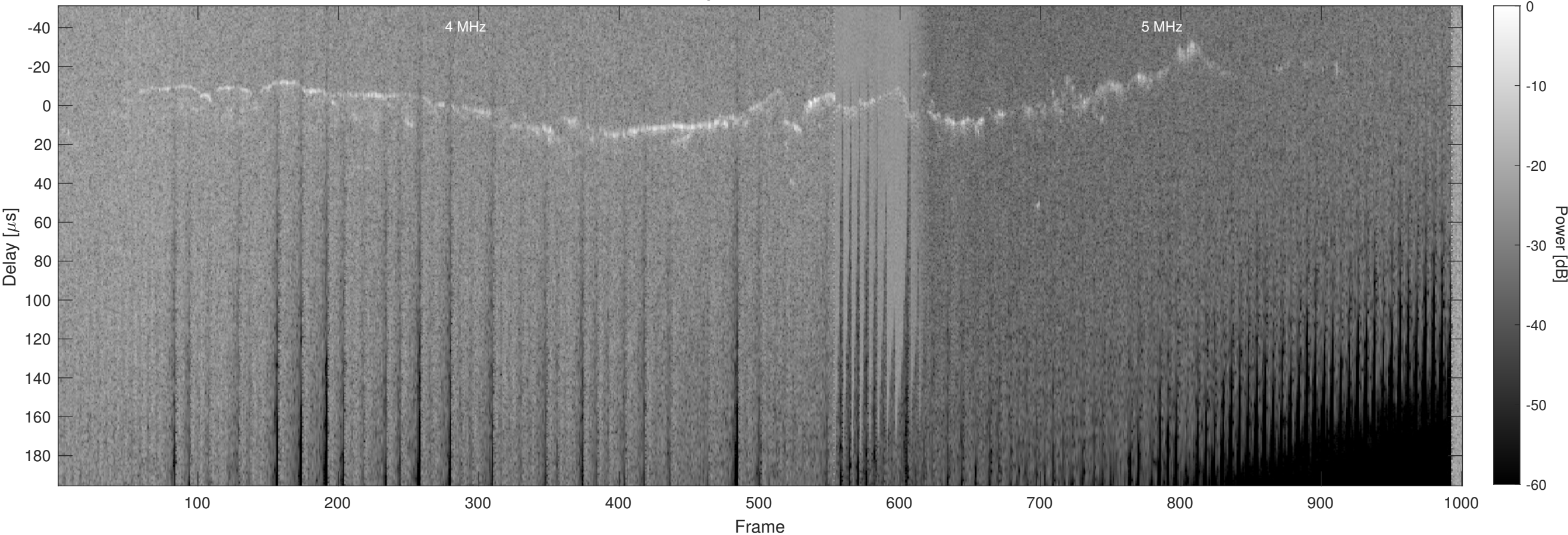
Orbit 12751, Chapman, No Window, Channel 2
