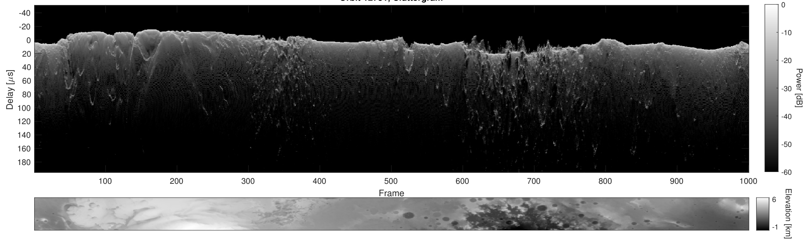
Orbit 12751, Cluttergram
