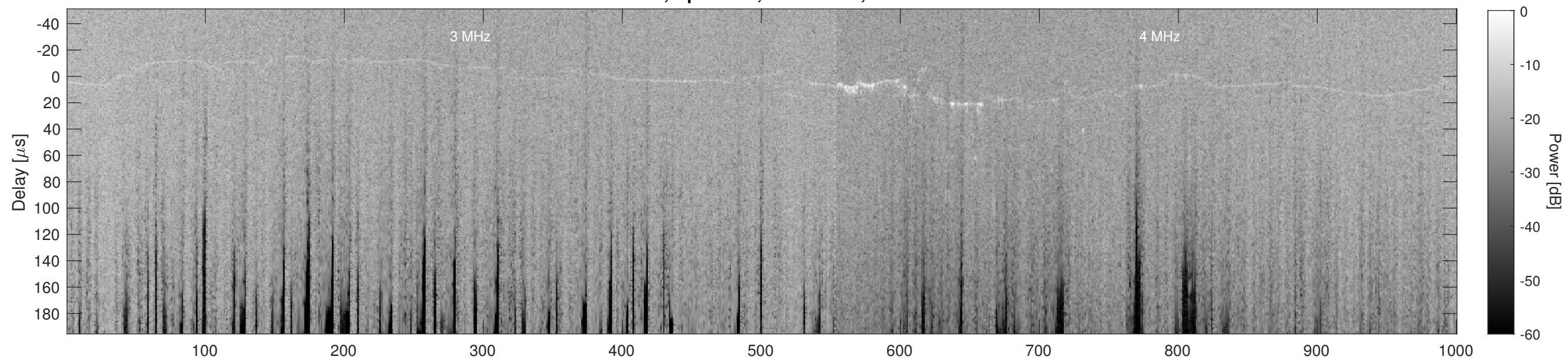
Orbit 12751, Cluttergram
