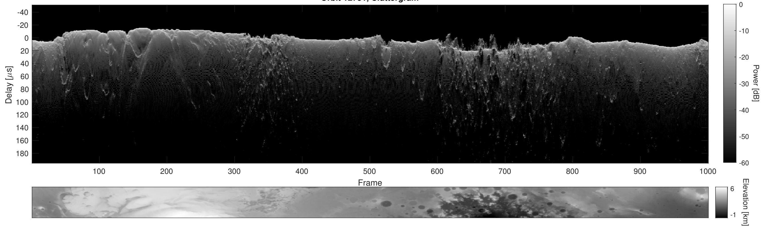
Orbit 12751, Cluttergram
