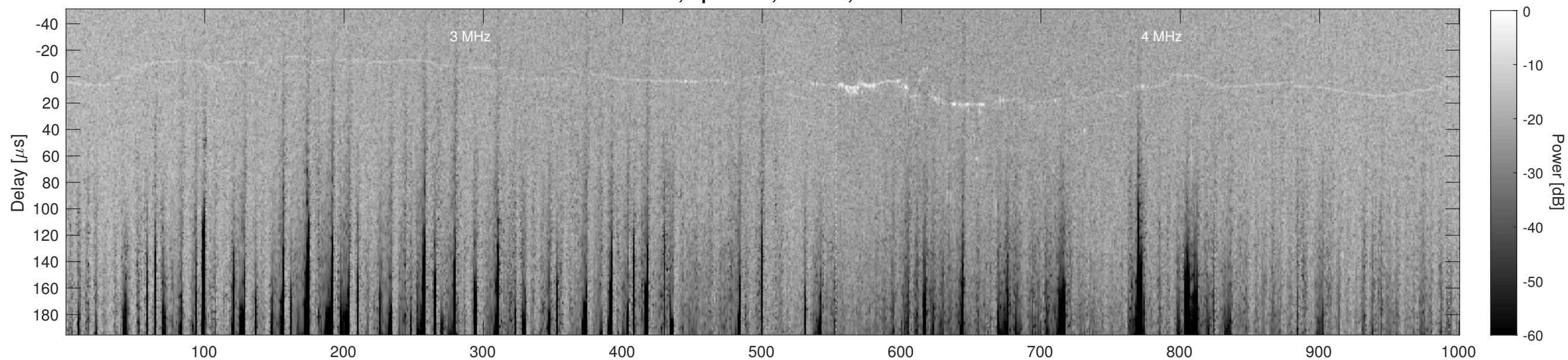
Orbit 12751, Cluttergram
