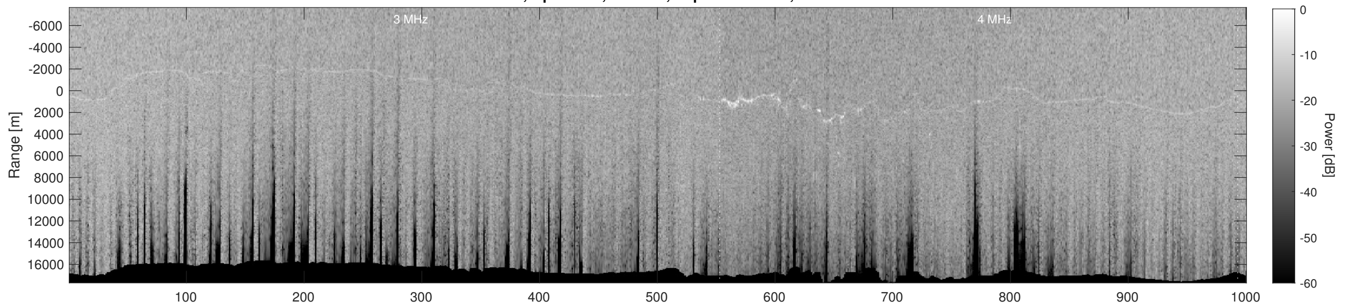
Orbit 12751, Depth-Corrected Cluttergram
