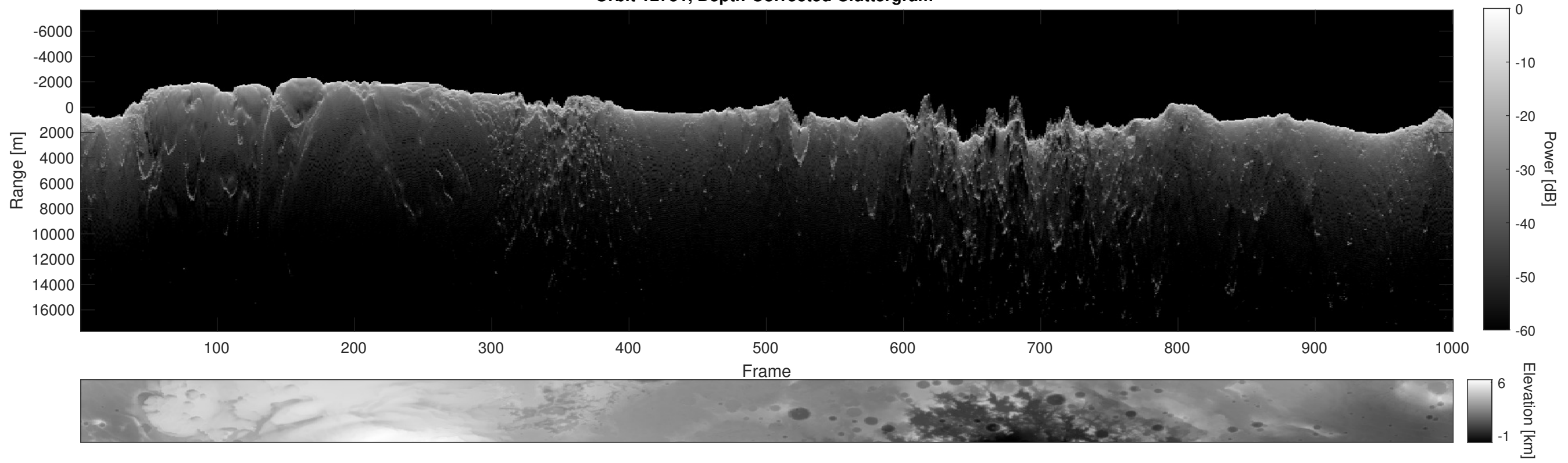
Orbit 12751, Depth-Corrected Cluttergram
