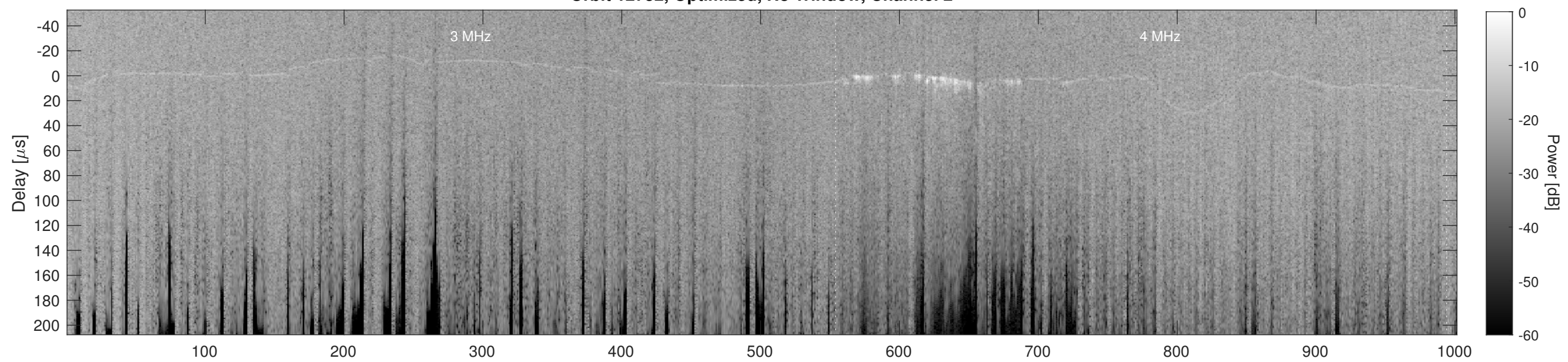
Orbit 12752, Cluttergram
