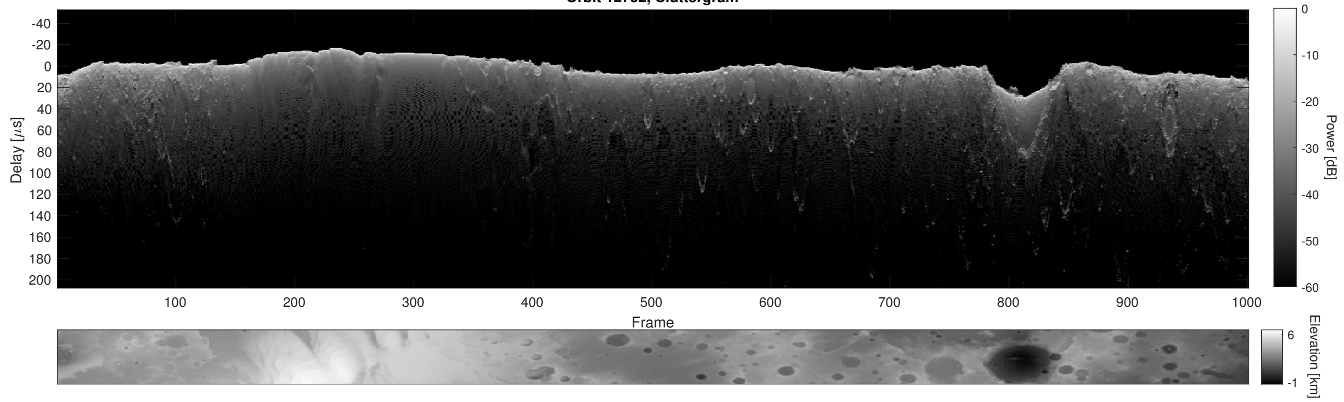
Orbit 12752, Cluttergram
