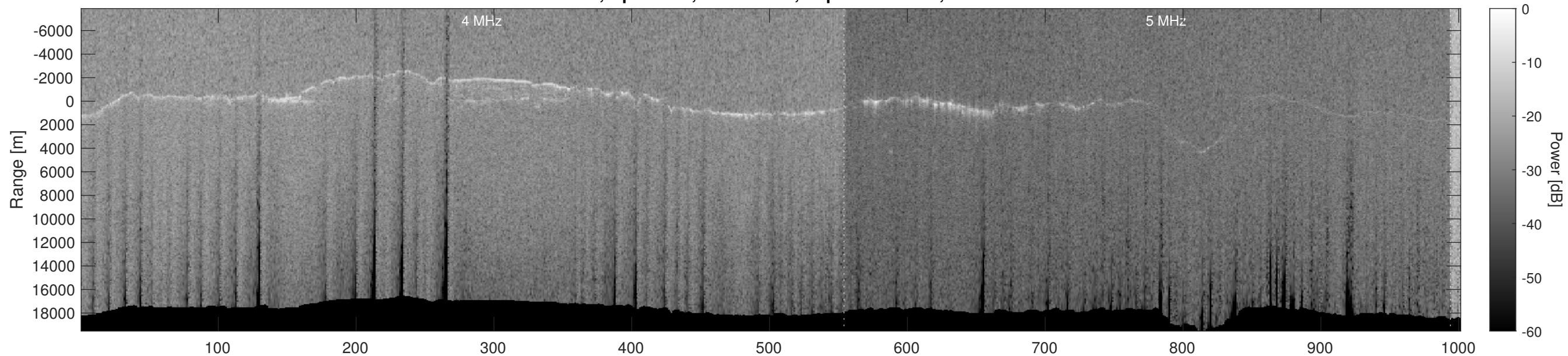
Orbit 12752, Optimized, No Window, Depth-Corrected, Channel 2
