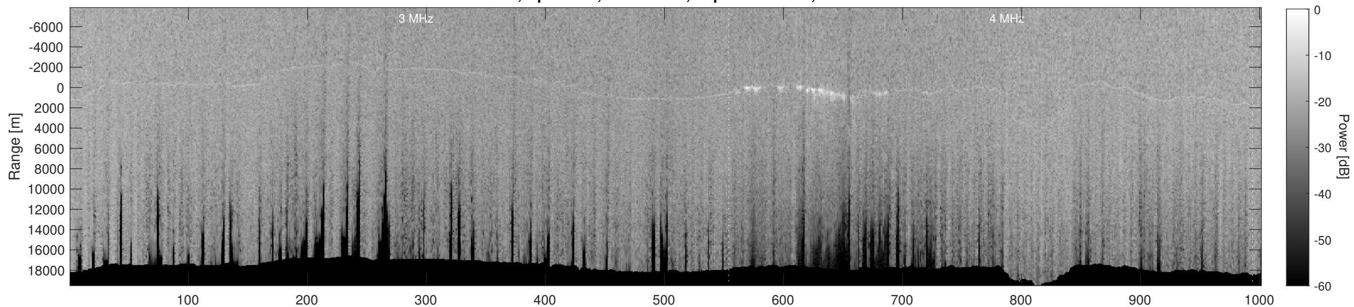
Orbit 12752, Depth-Corrected Cluttergram
