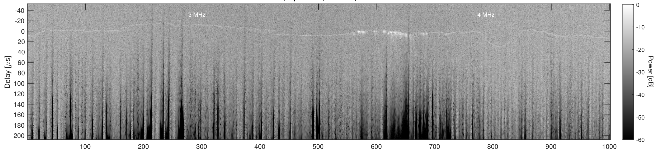
Orbit 12752, Cluttergram
