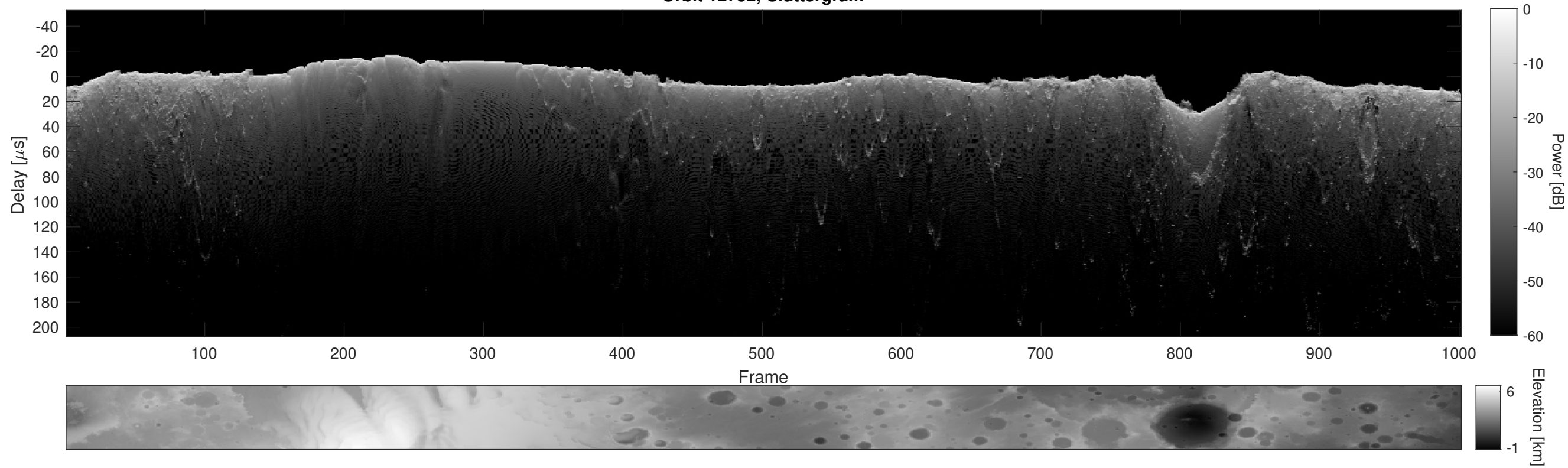
Orbit 12752, Cluttergram
