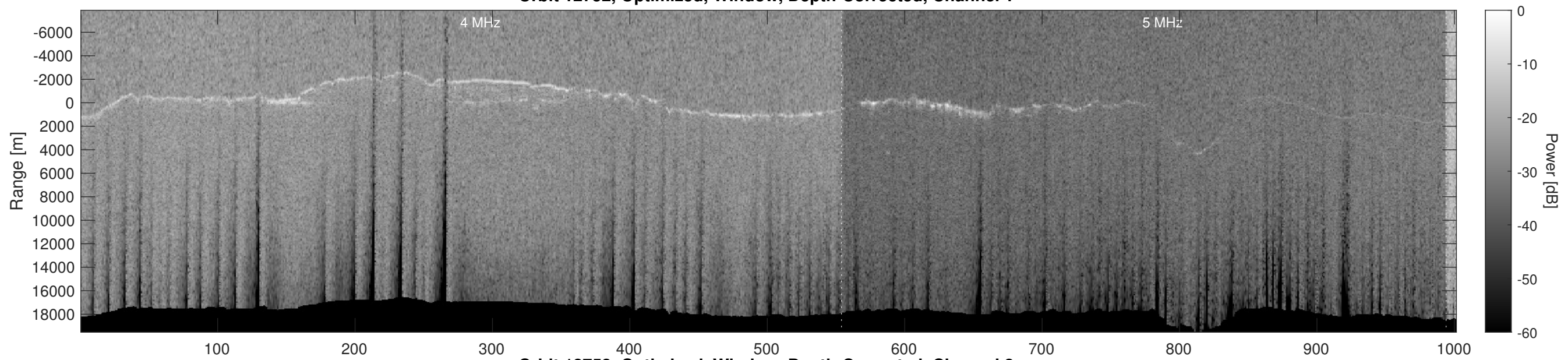
Orbit 12752, Optimized, Window, Depth-Corrected, Channel 2
