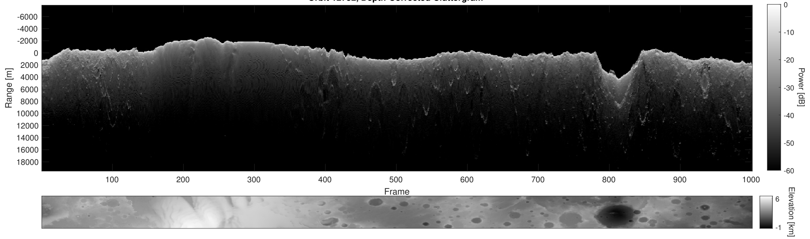
Orbit 12752, Depth-Corrected Cluttergram
