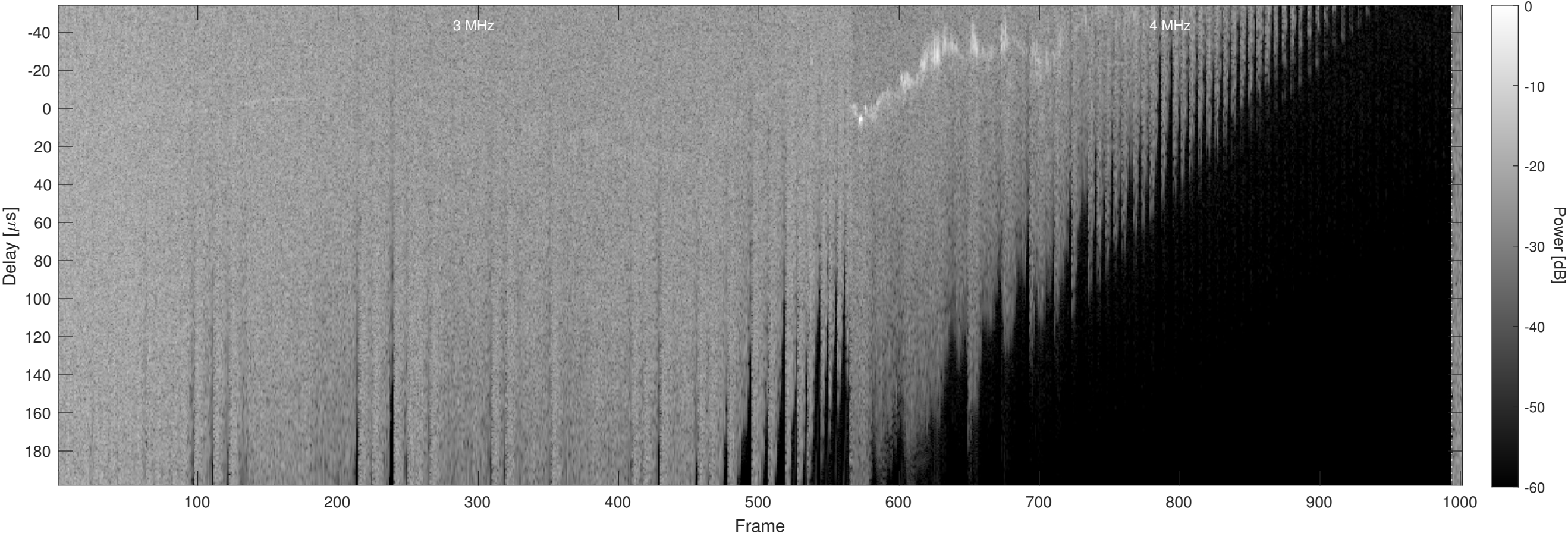
Orbit 12754, Chapman, No Window, Channel 2
